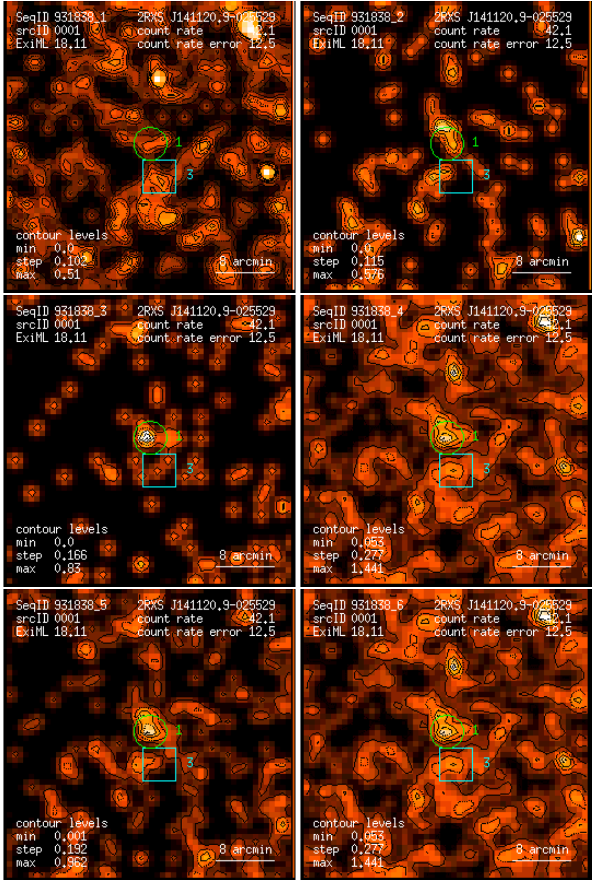
Figure 1: RASS 931838: detection 0001: band rate images, Gaussian filter: (1) PSPC channels 11 – 41, (2) 52 – 90, (3) 91 – 201, (4) 11 – 235, (5) 52 – 201, (6) 11 – 201. Broad band rates in counts/ks. Band rate contour levels in counts/ks/arcmin 2 .
