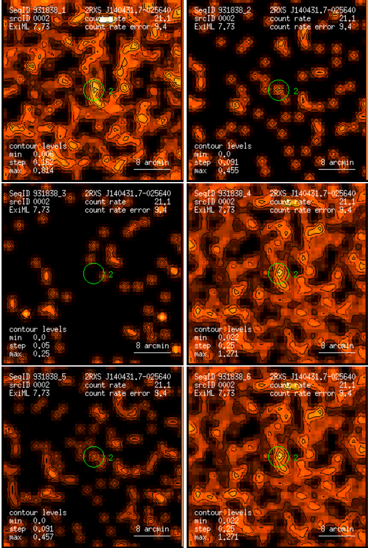
Figure 2: RASS 931838: detection 0002: band rate images, Gaussian filter: (1) PSPC channels 11 – 41, (2) 52 – 90, (3) 91 – 201, (4) 11 – 235, (5) 52 – 201, (6) 11 – 201. Broad band rates in counts/ks. Band rate contour levels in counts/ks/arcmin 2 .
