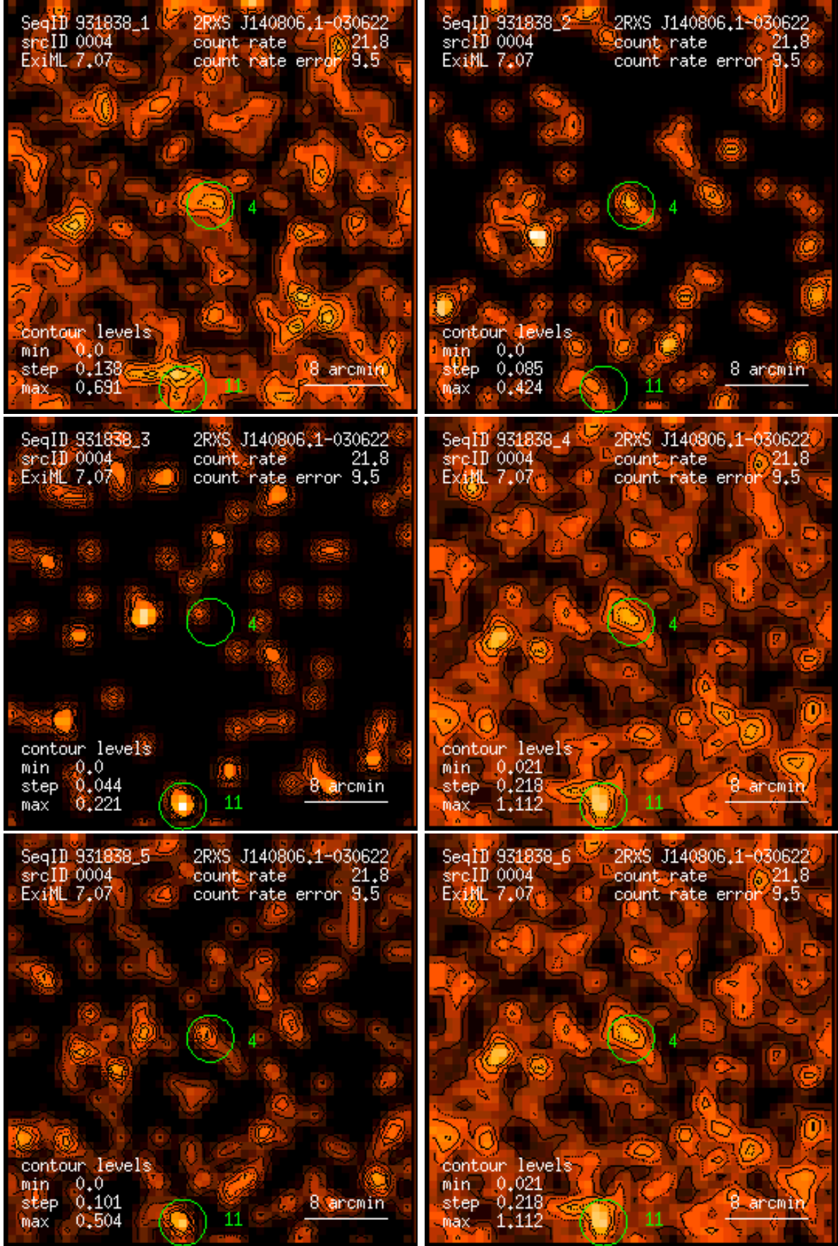
Figure 4: RASS 931838: detection 0004: band rate images, Gaussian filter: (1) PSPC channels 11 – 41, (2) 52 – 90, (3) 91 – 201, (4) 11 – 235, (5) 52 – 201, (6) 11 – 201. Broad band rates in counts/ks. Band rate contour levels in counts/ks/arcmin 2 .
