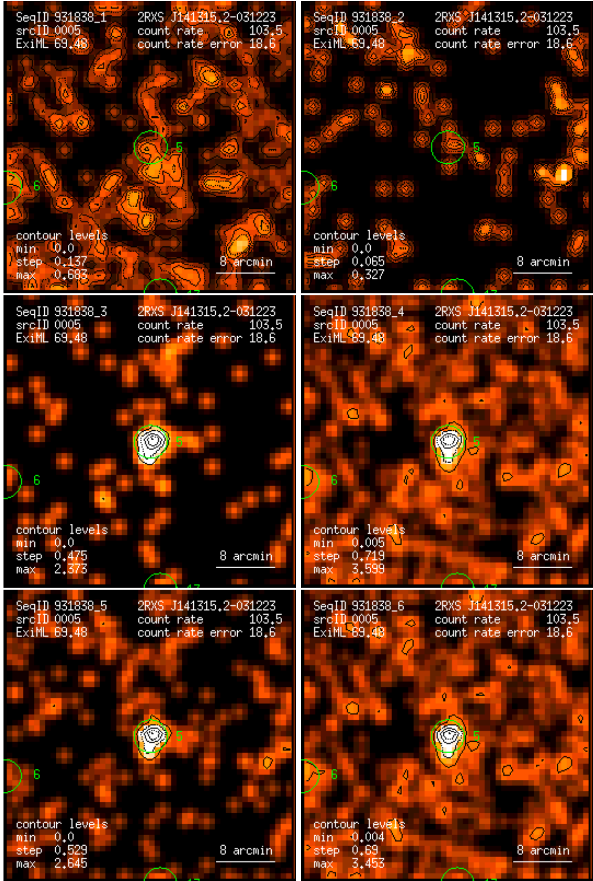
Figure 5: RASS 931838: detection 0005: band rate images, Gaussian filter: (1) PSPC channels 11 – 41, (2) 52 – 90, (3) 91 – 201, (4) 11 – 235, (5) 52 – 201, (6) 11 – 201. Broad band rates in counts/ks. Band rate contour levels in counts/ks/arcmin 2 .
