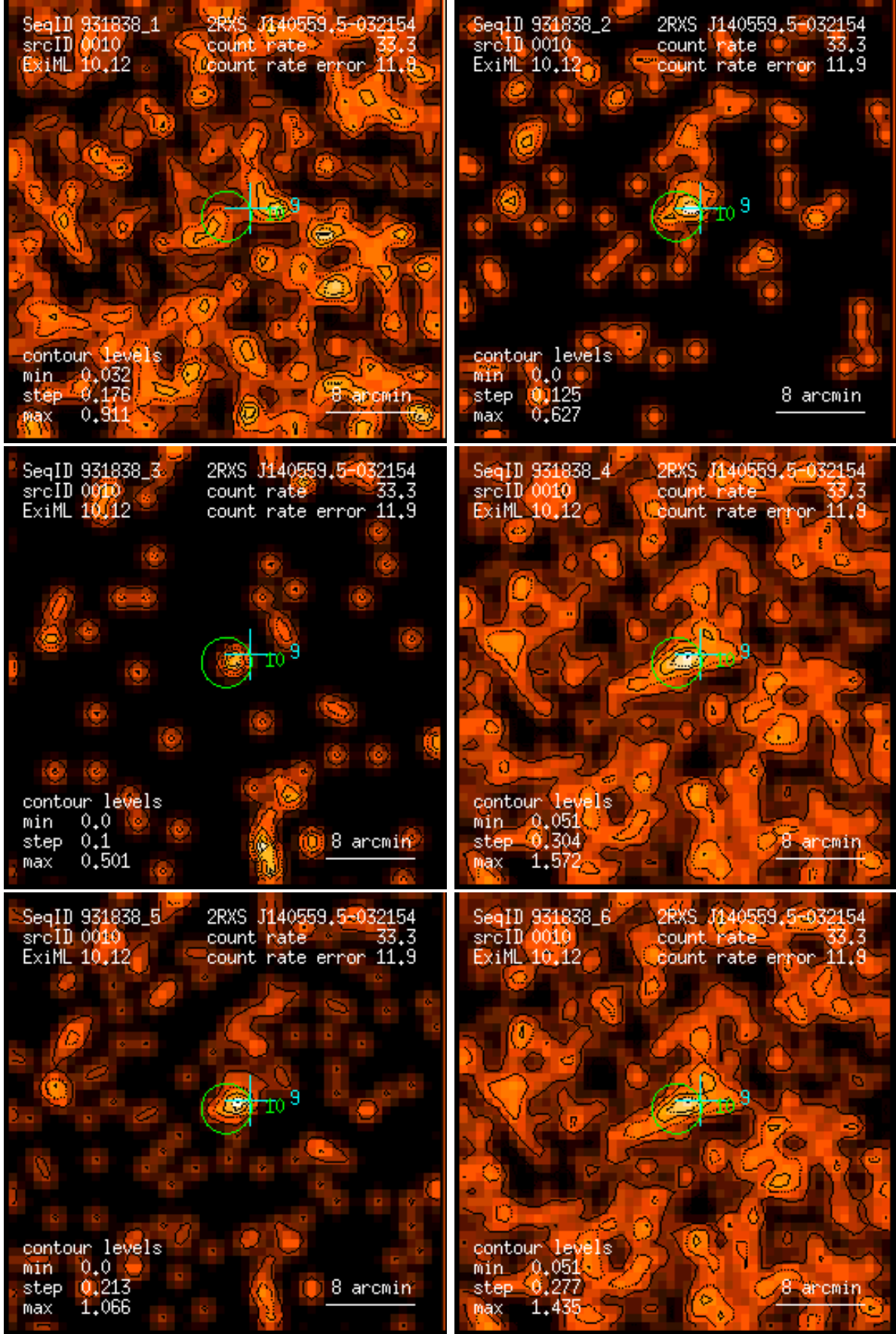
Figure 10: RASS 931838: detection 0010: band rate images, Gaussian filter: (1) PSPC channels 11 – 41, (2) 52 – 90, (3) 91 – 201, (4) 11 – 235, (5) 52 – 201, (6) 11 – 201. Broad band rates in counts/ks. Band rate contour levels in counts/ks/arcmin 2 .
