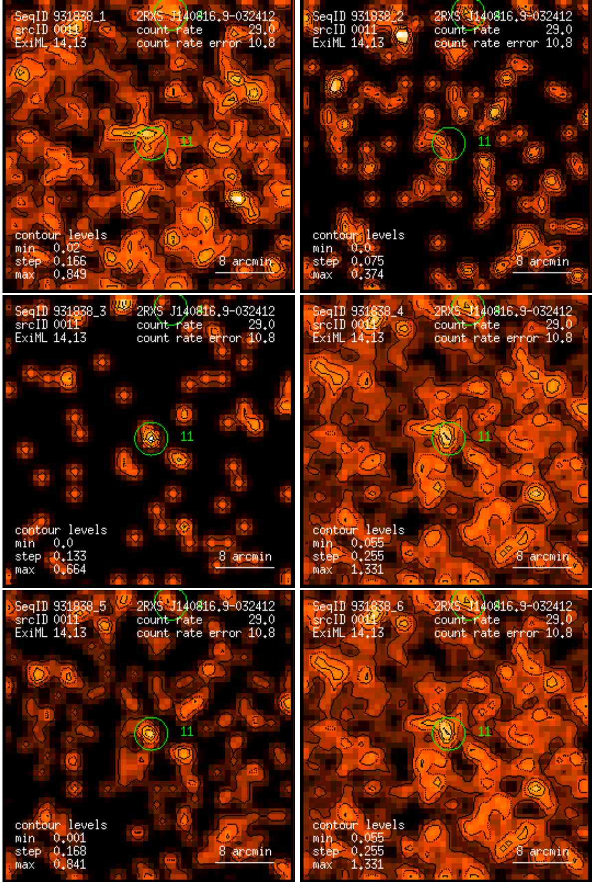
Figure 11: RASS 931838: detection 0011: band rate images, Gaussian filter: (1) PSPC channels 11 – 41, (2) 52 – 90, (3) 91 – 201, (4) 11 – 235, (5) 52 – 201, (6) 11 – 201. Broad band rates in counts/ks. Band rate contour levels in counts/ks/arcmin 2 .
