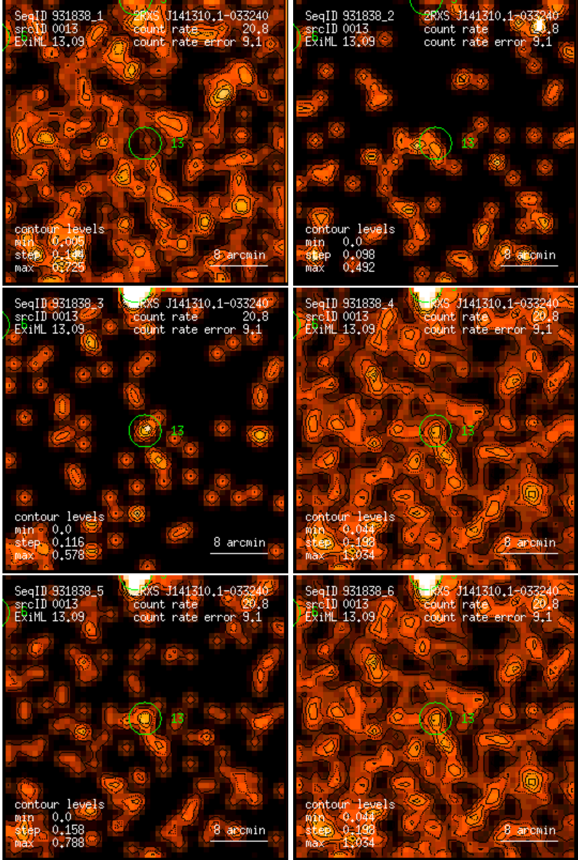
Figure 13: RASS 931838: detection 0013: band rate images, Gaussian filter: (1) PSPC channels 11 – 41, (2) 52 – 90, (3) 91 – 201, (4) 11 – 235, (5) 52 – 201, (6) 11 – 201. Broad band rates in counts/ks. Band rate contour levels in counts/ks/arcmin 2 .
