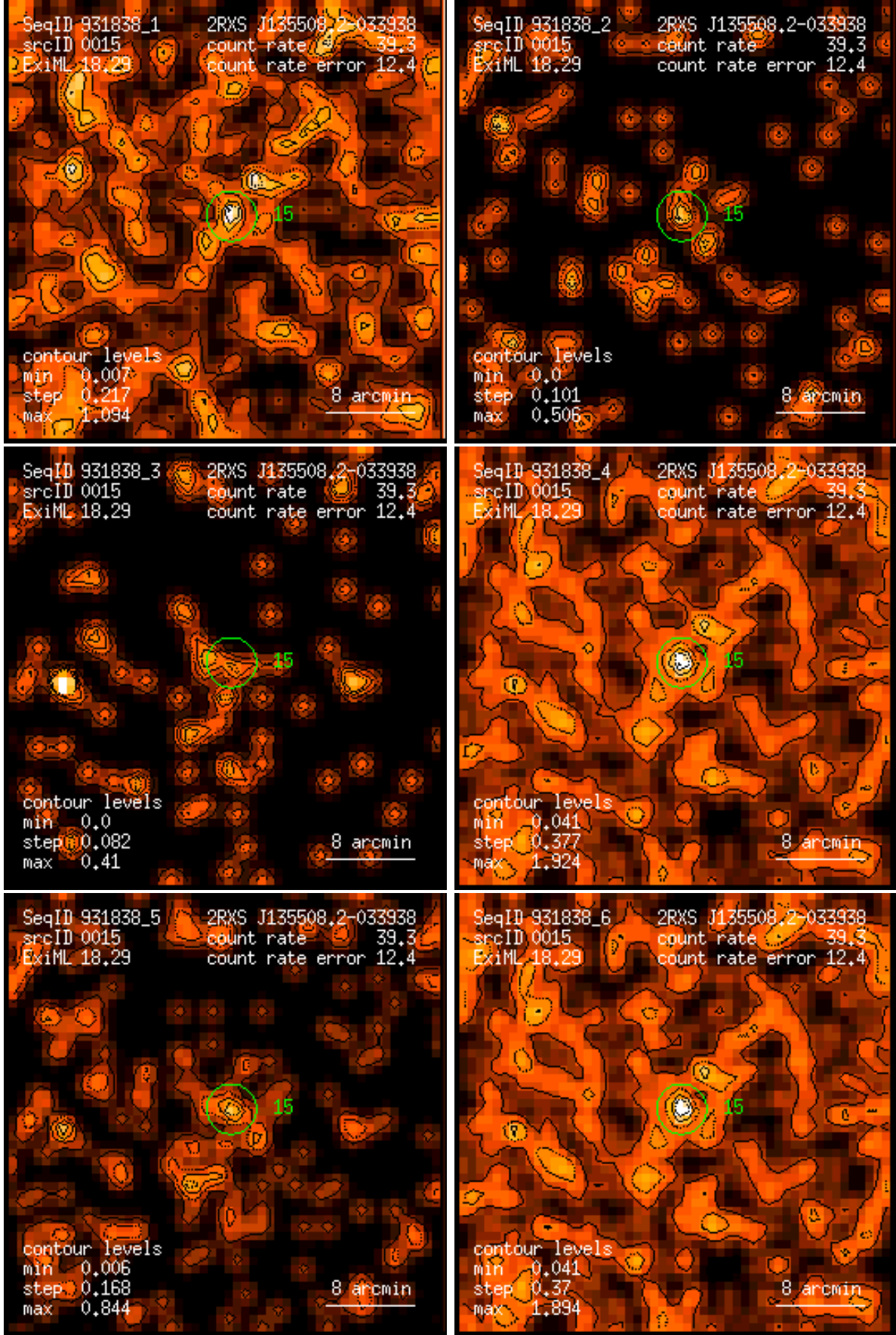
Figure 15: RASS 931838: detection 0015: band rate images, Gaussian filter: (1) PSPC channels 11 – 41, (2) 52 – 90, (3) 91 – 201, (4) 11 – 235, (5) 52 – 201, (6) 11 – 201. Broad band rates in counts/ks. Band rate contour levels in counts/ks/arcmin 2 .
