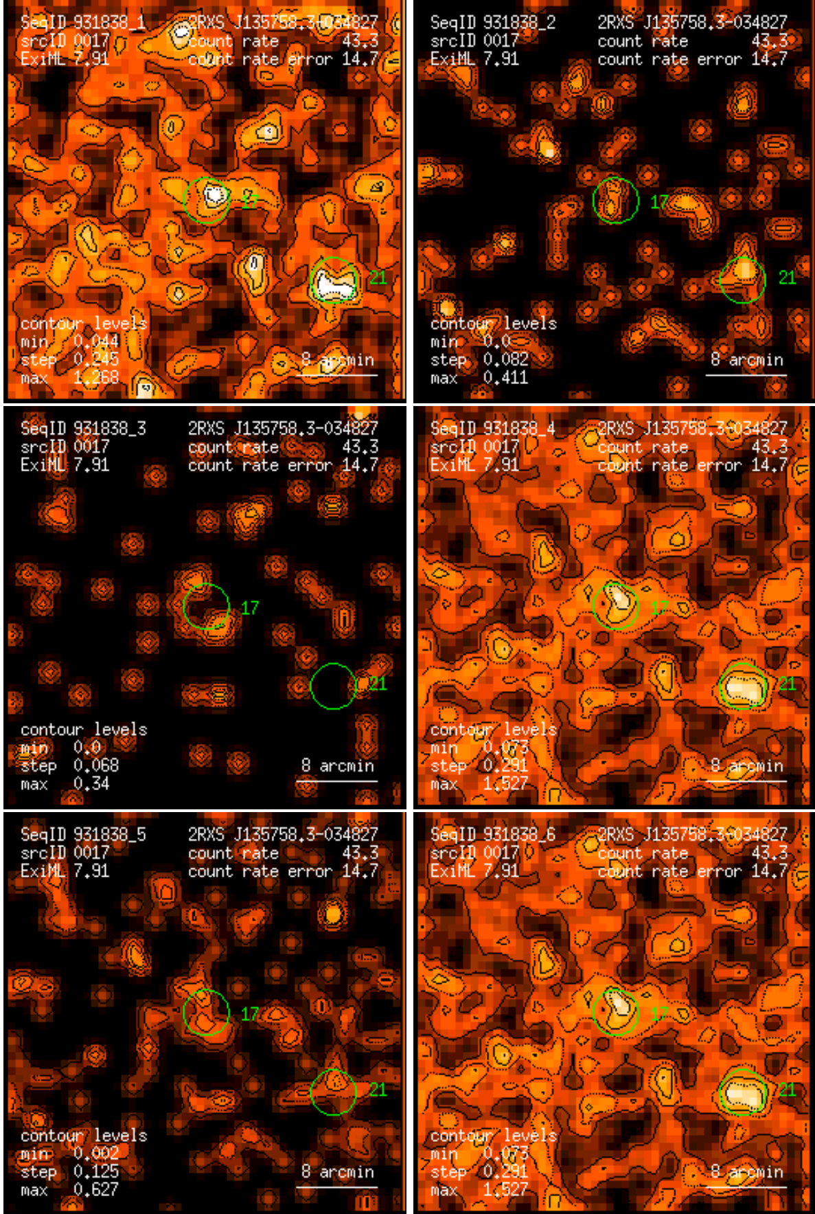
Figure 17: RASS 931838: detection 0017: band rate images, Gaussian filter: (1) PSPC channels 11 – 41, (2) 52 – 90, (3) 91 – 201, (4) 11 – 235, (5) 52 – 201, (6) 11 – 201. Broad band rates in counts/ks. Band rate contour levels in counts/ks/arcmin 2 .
