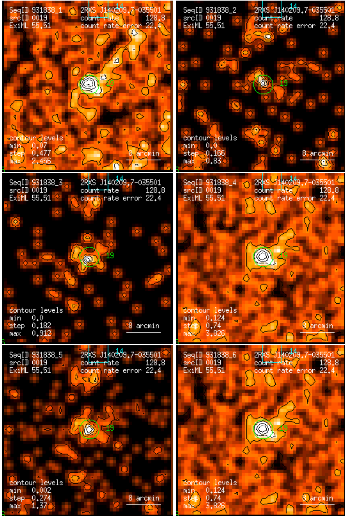
Figure 19: RASS 931838: detection 0019: band rate images, Gaussian filter: (1) PSPC channels 11 – 41, (2) 52 – 90, (3) 91 – 201, (4) 11 – 235, (5) 52 – 201, (6) 11 – 201. Broad band rates in counts/ks. Band rate contour levels in counts/ks/arcmin 2 .
