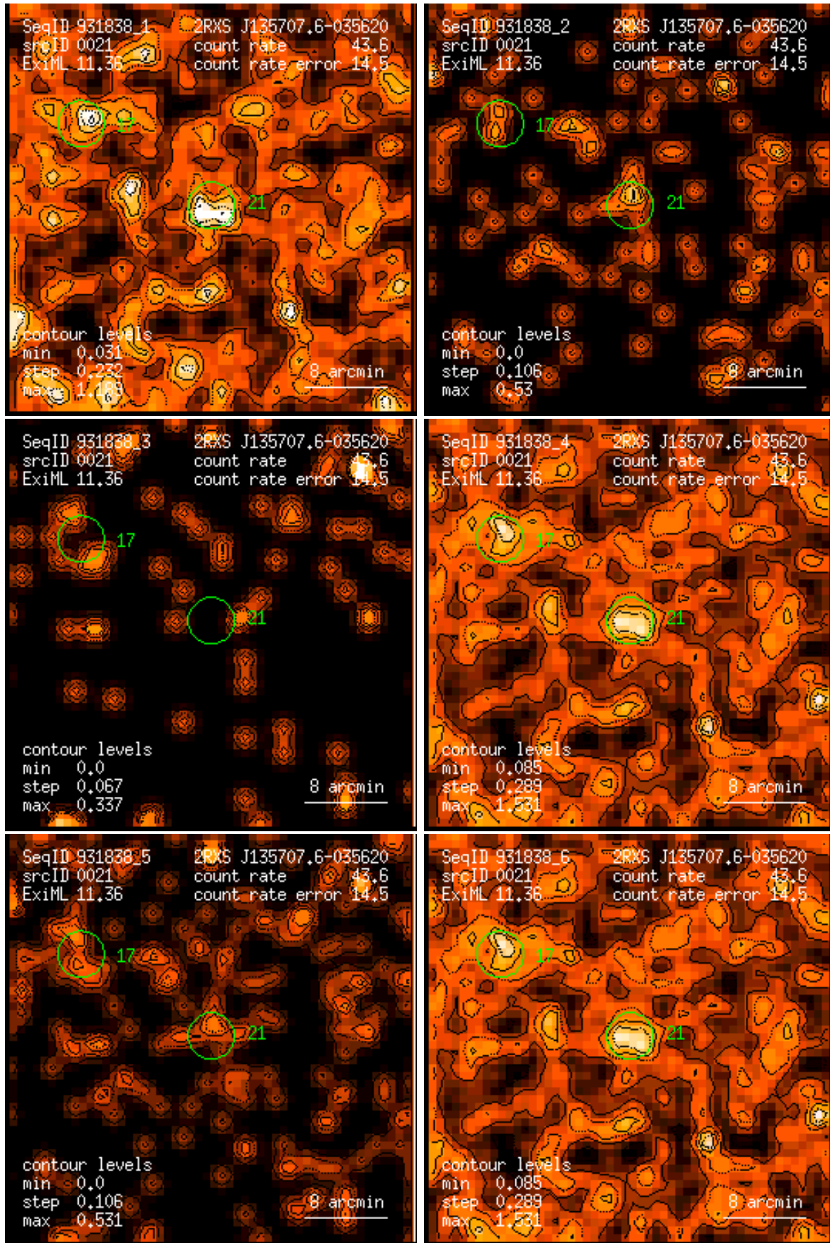
Figure 21: RASS 931838: detection 0021: band rate images, Gaussian filter: (1) PSPC channels 11 – 41, (2) 52 – 90, (3) 91 – 201, (4) 11 – 235, (5) 52 – 201, (6) 11 – 201. Broad band rates in counts/ks. Band rate contour levels in counts/ks/arcmin 2 .
