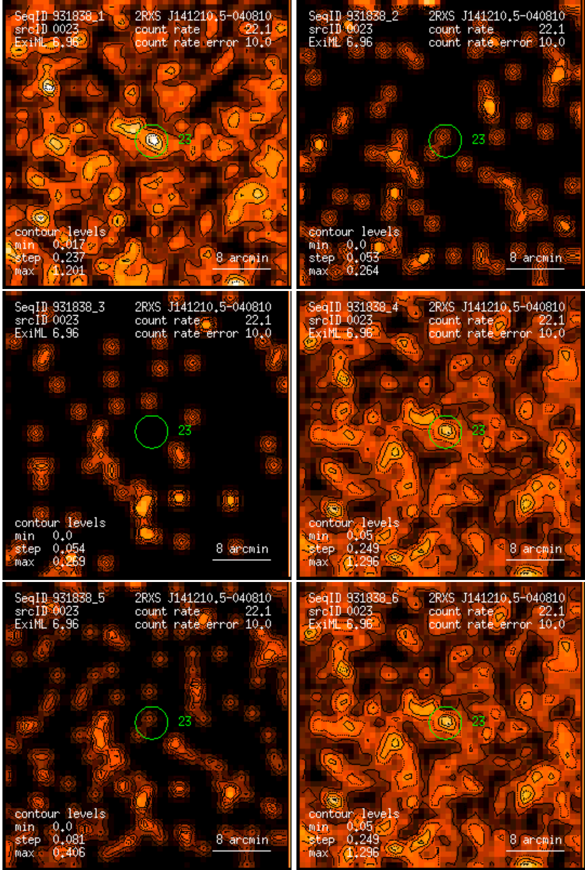
Figure 23: RASS 931838: detection 0023: band rate images, Gaussian filter: (1) PSPC channels 11 – 41, (2) 52 – 90, (3) 91 – 201, (4) 11 – 235, (5) 52 – 201, (6) 11 – 201. Broad band rates in counts/ks. Band rate contour levels in counts/ks/arcmin 2 .
