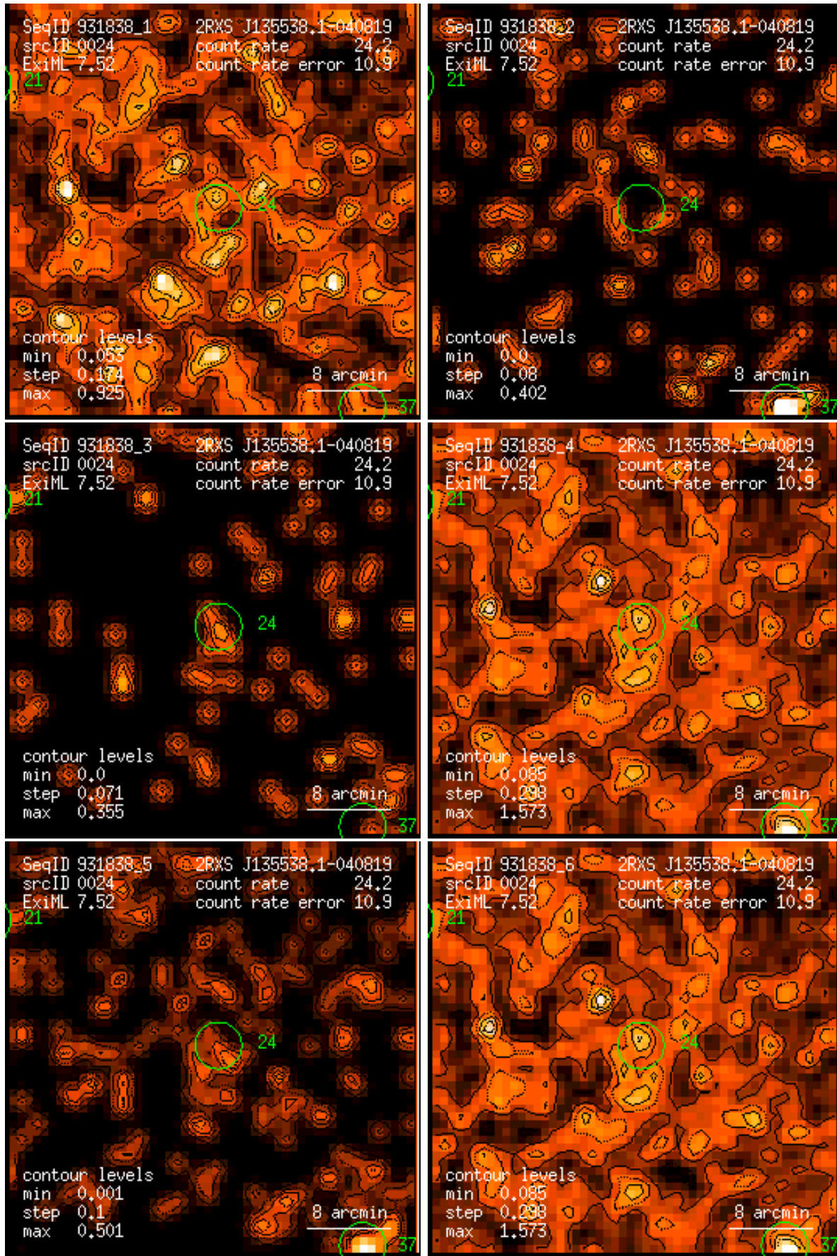
Figure 24: RASS 931838: detection 0024: band rate images, Gaussian filter: (1) PSPC channels 11 – 41, (2) 52 – 90, (3) 91 – 201, (4) 11 – 235, (5) 52 – 201, (6) 11 – 201. Broad band rates in counts/ks. Band rate contour levels in counts/ks/arcmin 2 .
