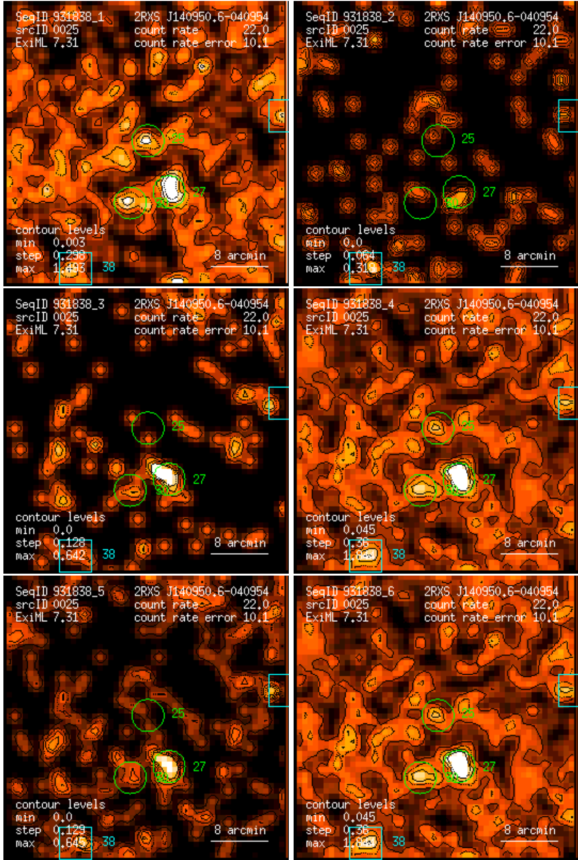
Figure 25: RASS 931838: detection 0025: band rate images, Gaussian filter: (1) PSPC channels 11 – 41, (2) 52 – 90, (3) 91 – 201, (4) 11 – 235, (5) 52 – 201, (6) 11 – 201. Broad band rates in counts/ks. Band rate contour levels in counts/ks/arcmin 2 .
