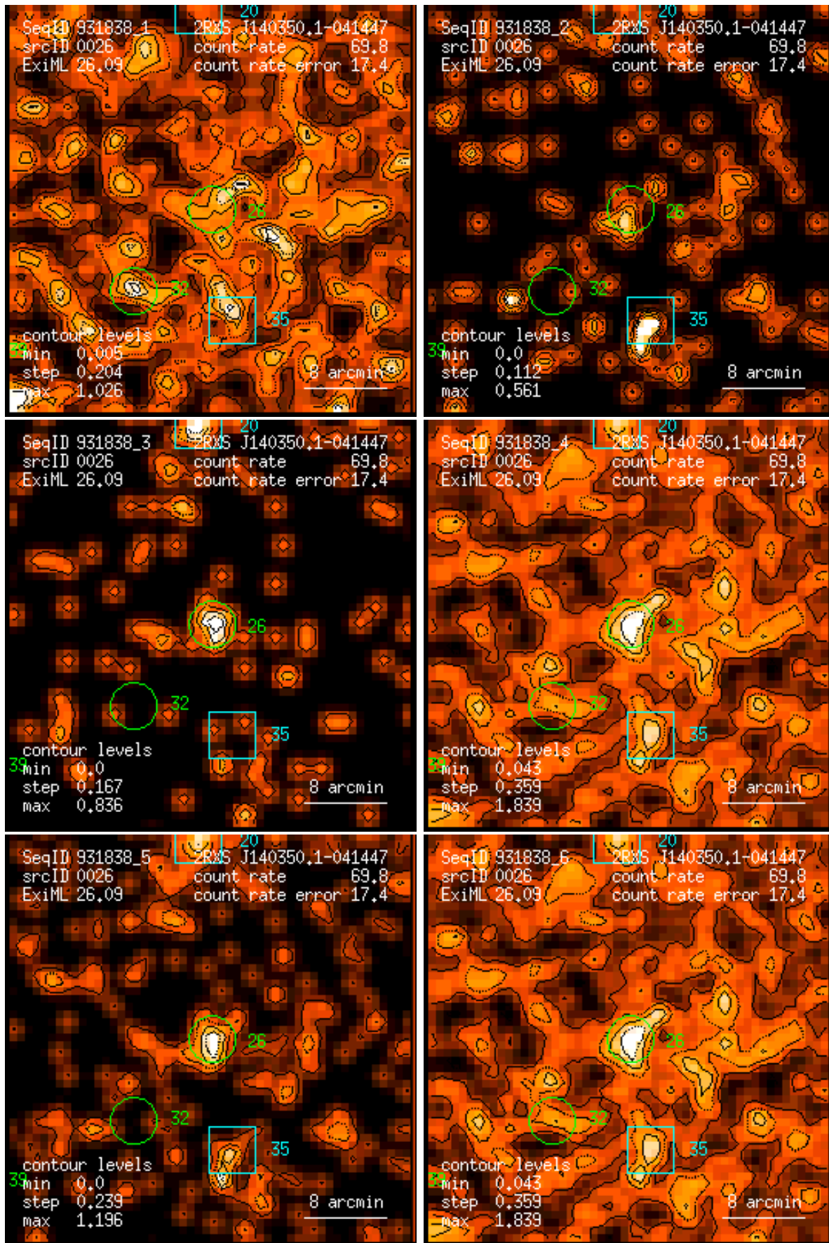
Figure 26: RASS 931838: detection 0026: band rate images, Gaussian filter: (1) PSPC channels 11 – 41, (2) 52 – 90, (3) 91 – 201, (4) 11 – 235, (5) 52 – 201, (6) 11 – 201. Broad band rates in counts/ks. Band rate contour levels in counts/ks/arcmin 2 .
