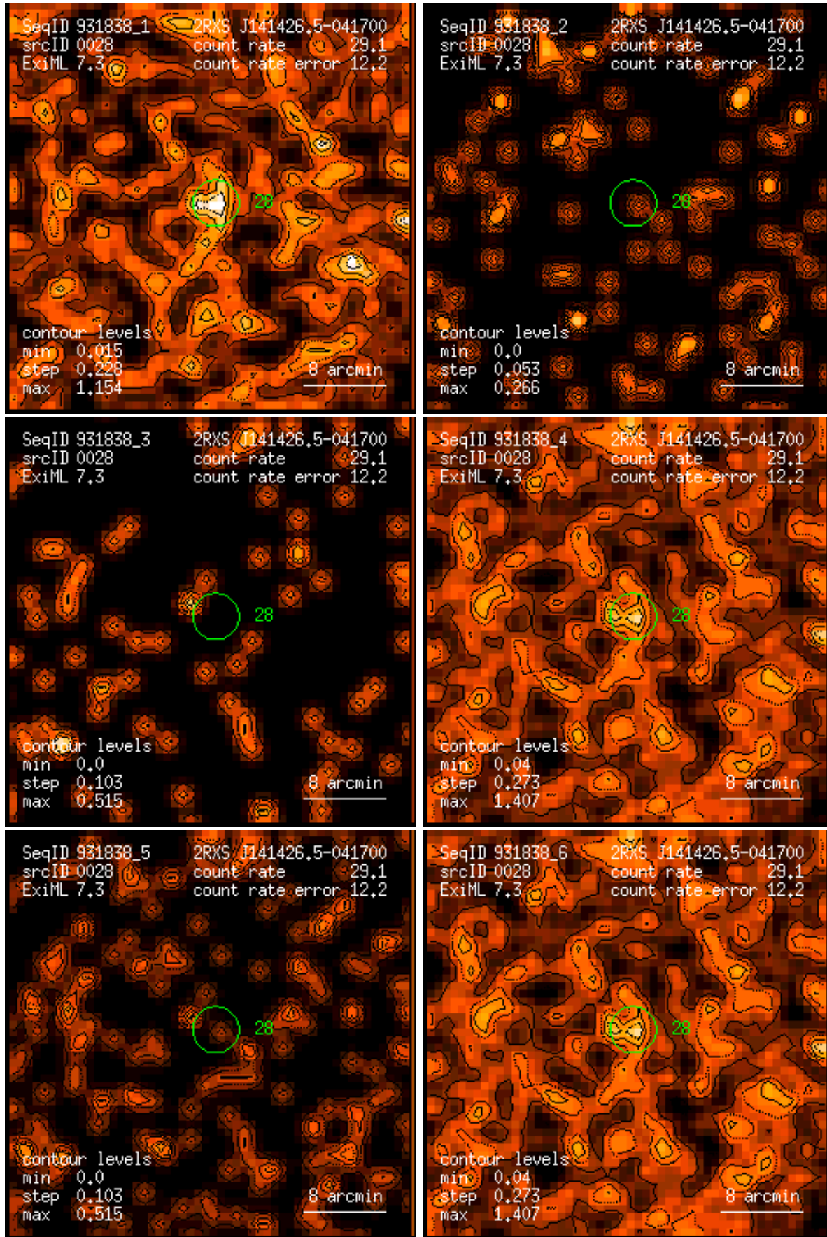
Figure 28: RASS 931838: detection 0028: band rate images, Gaussian filter: (1) PSPC channels 11 – 41, (2) 52 – 90, (3) 91 – 201, (4) 11 – 235, (5) 52 – 201, (6) 11 – 201. Broad band rates in counts/ks. Band rate contour levels in counts/ks/arcmin 2 .
