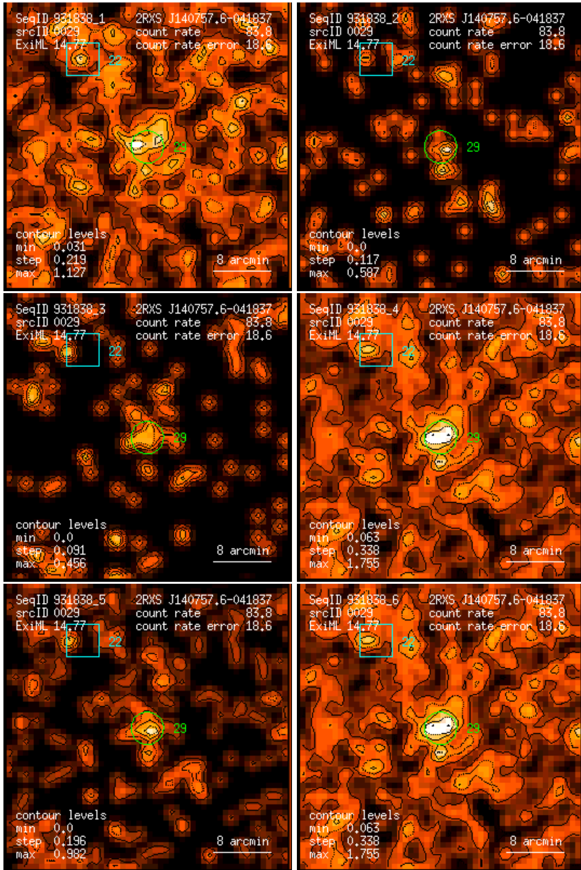
Figure 29: RASS 931838: detection 0029: band rate images, Gaussian filter: (1) PSPC channels 11 – 41, (2) 52 – 90, (3) 91 – 201, (4) 11 – 235, (5) 52 – 201, (6) 11 – 201. Broad band rates in counts/ks. Band rate contour levels in counts/ks/arcmin 2 .
