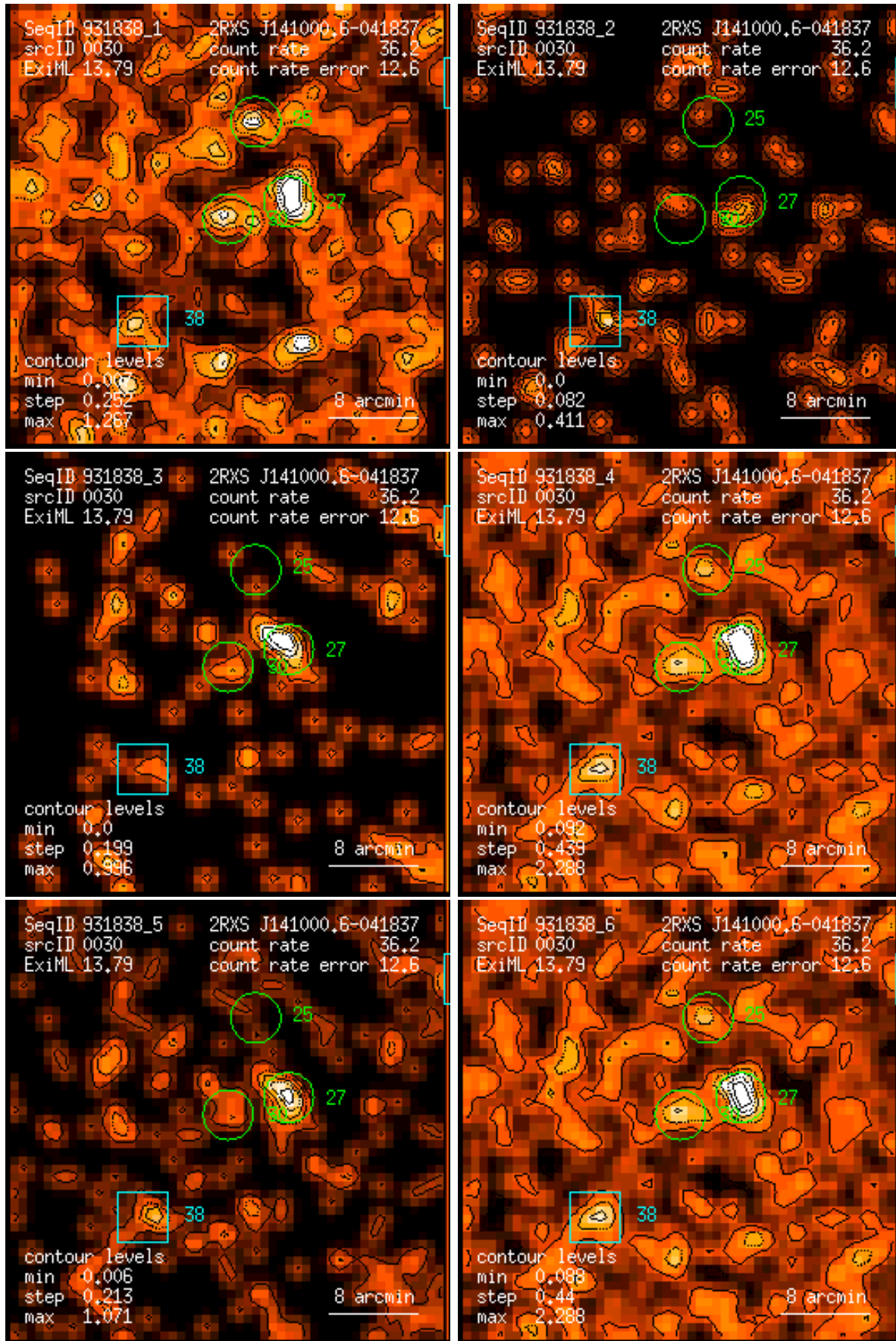
Figure 30: RASS 931838: detection 0030: band rate images, Gaussian filter: (1) PSPC channels 11 – 41, (2) 52 – 90, (3) 91 – 201, (4) 11 – 235, (5) 52 – 201, (6) 11 – 201. Broad band rates in counts/ks. Band rate contour levels in counts/ks/arcmin 2 .
