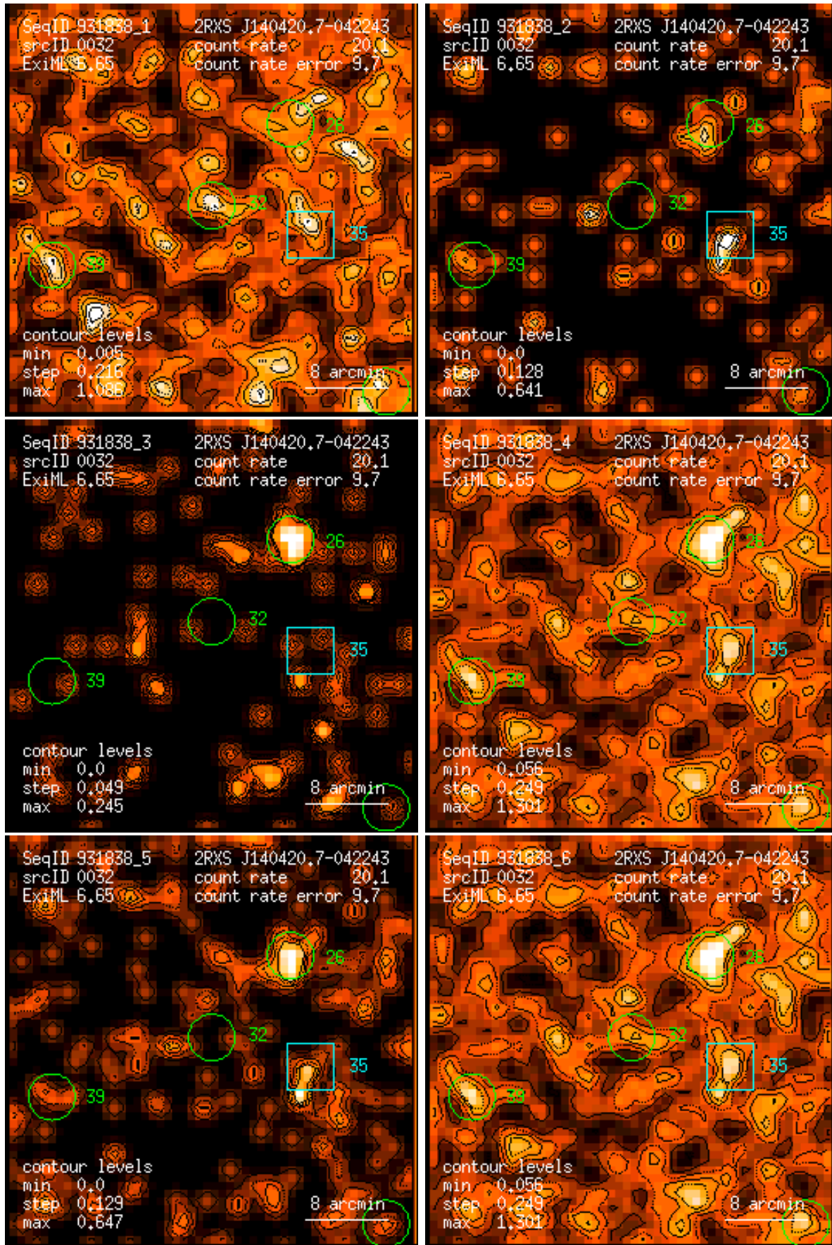
Figure 32: RASS 931838: detection 0032: band rate images, Gaussian filter: (1) PSPC channels 11 – 41, (2) 52 – 90, (3) 91 – 201, (4) 11 – 235, (5) 52 – 201, (6) 11 – 201. Broad band rates in counts/ks. Band rate contour levels in counts/ks/arcmin 2 .
