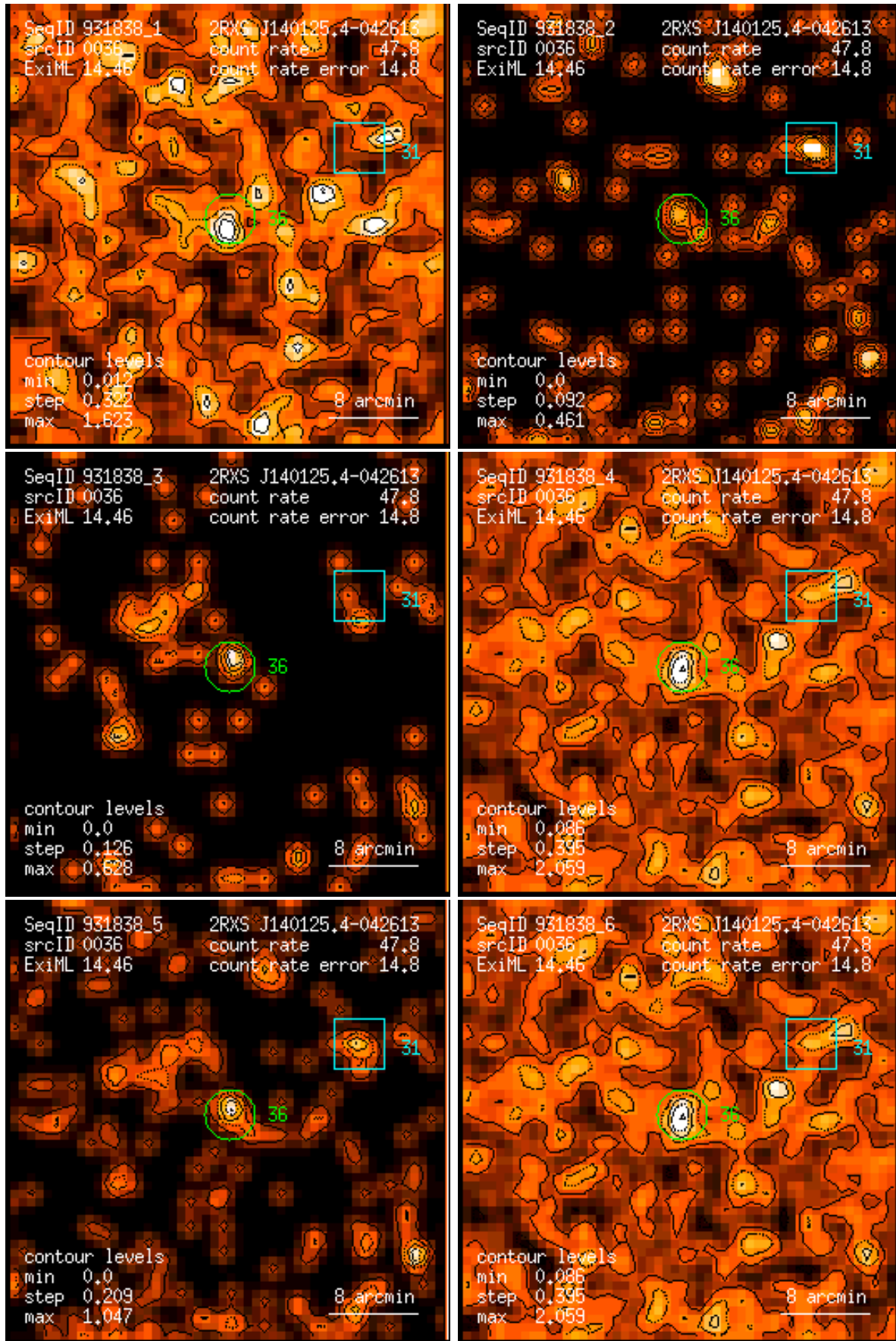
Figure 36: RASS 931838: detection 0036: band rate images, Gaussian filter: (1) PSPC channels 11 – 41, (2) 52 – 90, (3) 91 – 201, (4) 11 – 235, (5) 52 – 201, (6) 11 – 201. Broad band rates in counts/ks. Band rate contour levels in counts/ks/arcmin 2 .
