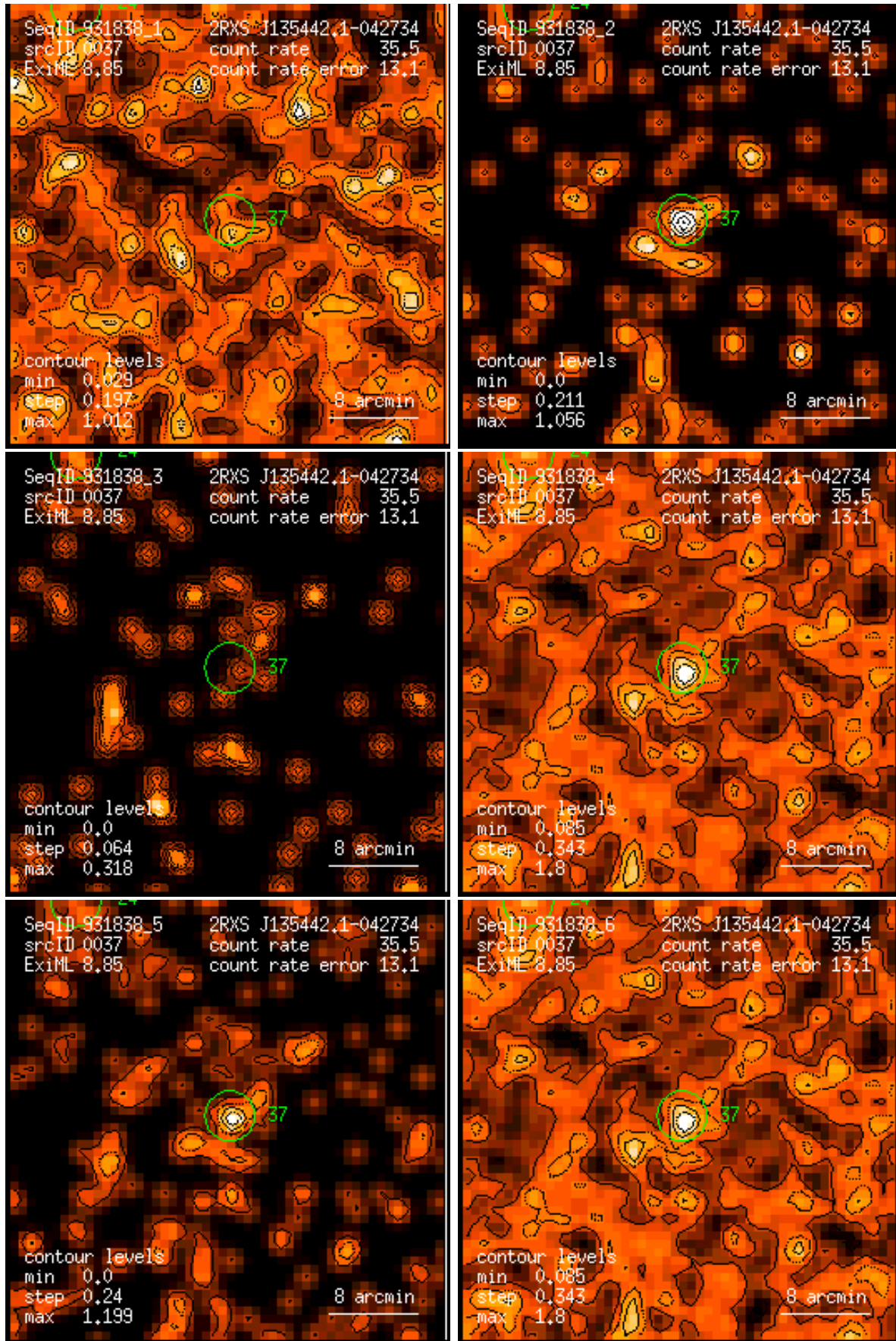
Figure 37: RASS 931838: detection 0037: band rate images, Gaussian filter: (1) PSPC channels 11 – 41, (2) 52 – 90, (3) 91 – 201, (4) 11 – 235, (5) 52 – 201, (6) 11 – 201. Broad band rates in counts/ks. Band rate contour levels in counts/ks/arcmin 2 .
