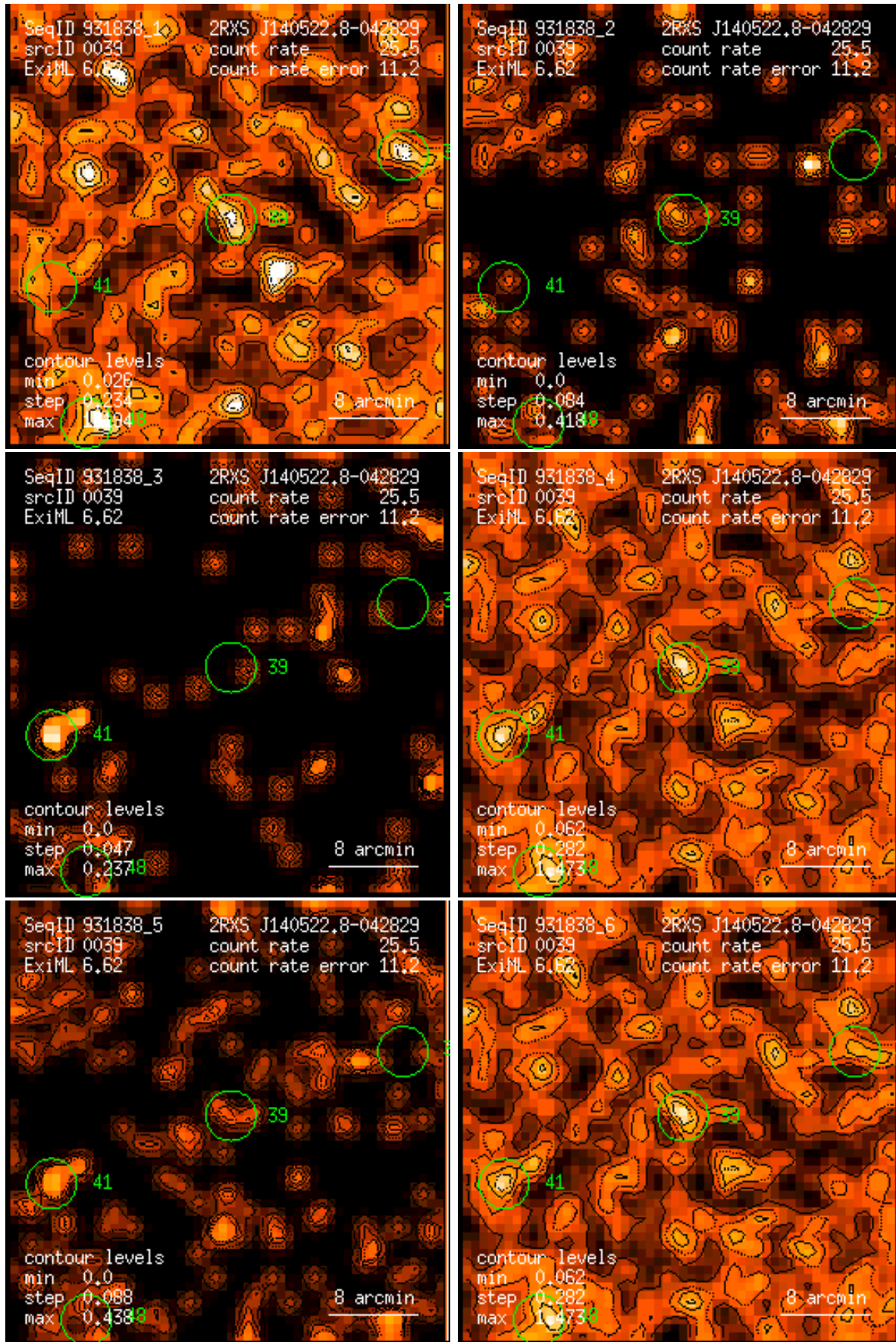
Figure 39: RASS 931838: detection 0039: band rate images, Gaussian filter: (1) PSPC channels 11 – 41, (2) 52 – 90, (3) 91 – 201, (4) 11 – 235, (5) 52 – 201, (6) 11 – 201. Broad band rates in counts/ks. Band rate contour levels in counts/ks/arcmin 2 .
