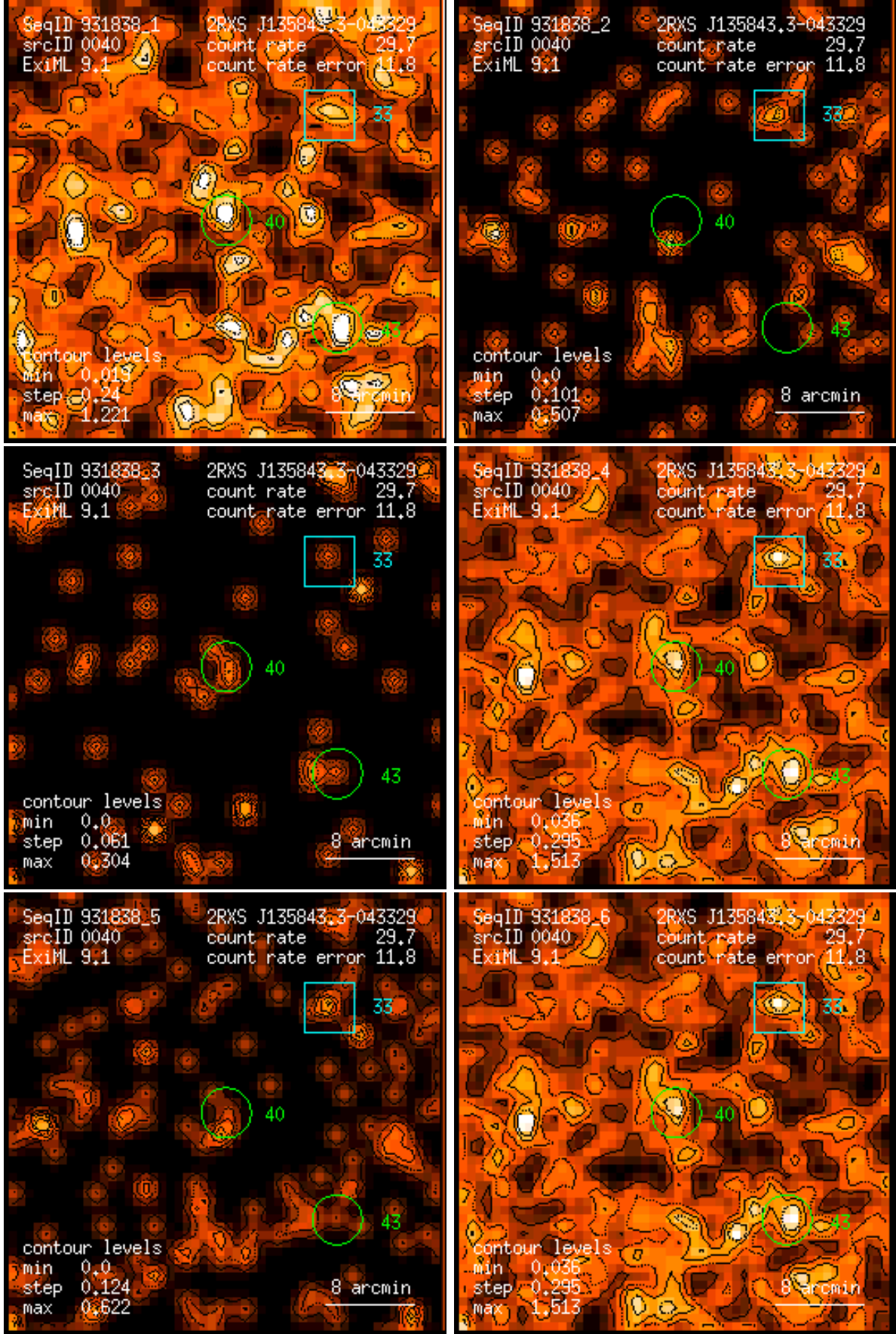
Figure 40: RASS 931838: detection 0040: band rate images, Gaussian filter: (1) PSPC channels 11 – 41, (2) 52 – 90, (3) 91 – 201, (4) 11 – 235, (5) 52 – 201, (6) 11 – 201. Broad band rates in counts/ks. Band rate contour levels in counts/ks/arcmin 2 .
