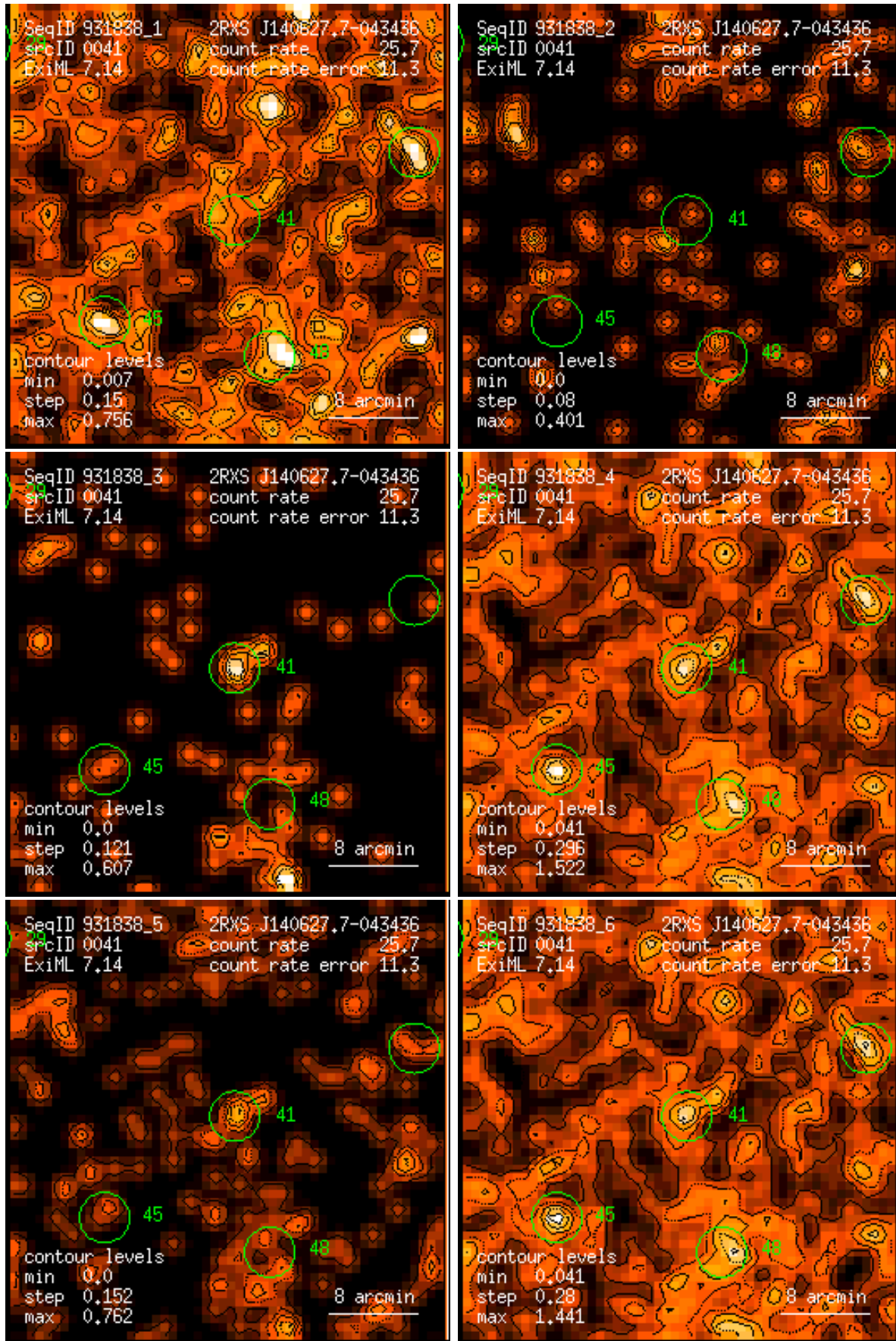
Figure 41: RASS 931838: detection 0041: band rate images, Gaussian filter: (1) PSPC channels 11 – 41, (2) 52 – 90, (3) 91 – 201, (4) 11 – 235, (5) 52 – 201, (6) 11 – 201. Broad band rates in counts/ks. Band rate contour levels in counts/ks/arcmin 2 .
