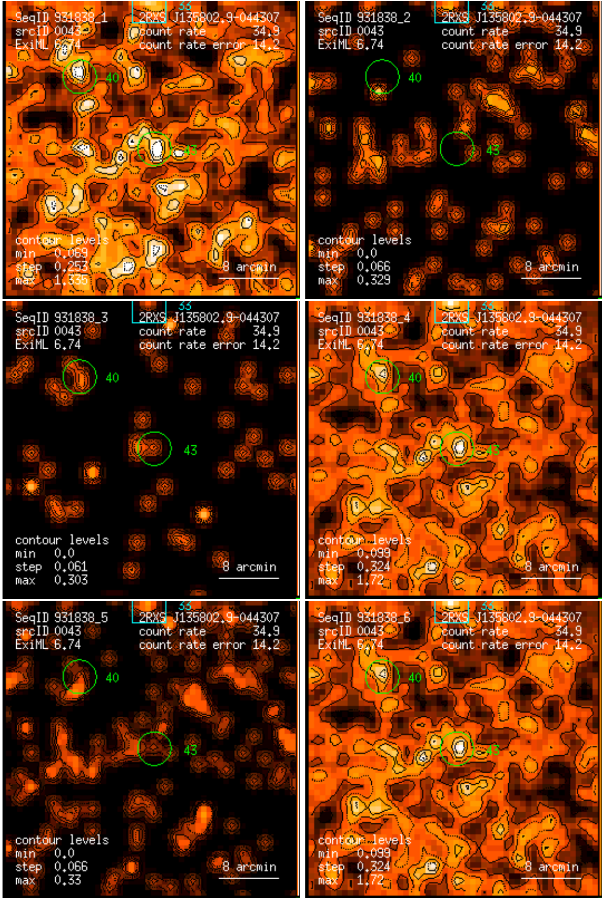
Figure 43: RASS 931838: detection 0043: band rate images, Gaussian filter: (1) PSPC channels 11 – 41, (2) 52 – 90, (3) 91 – 201, (4) 11 – 235, (5) 52 – 201, (6) 11 – 201. Broad band rates in counts/ks. Band rate contour levels in counts/ks/arcmin 2 .
