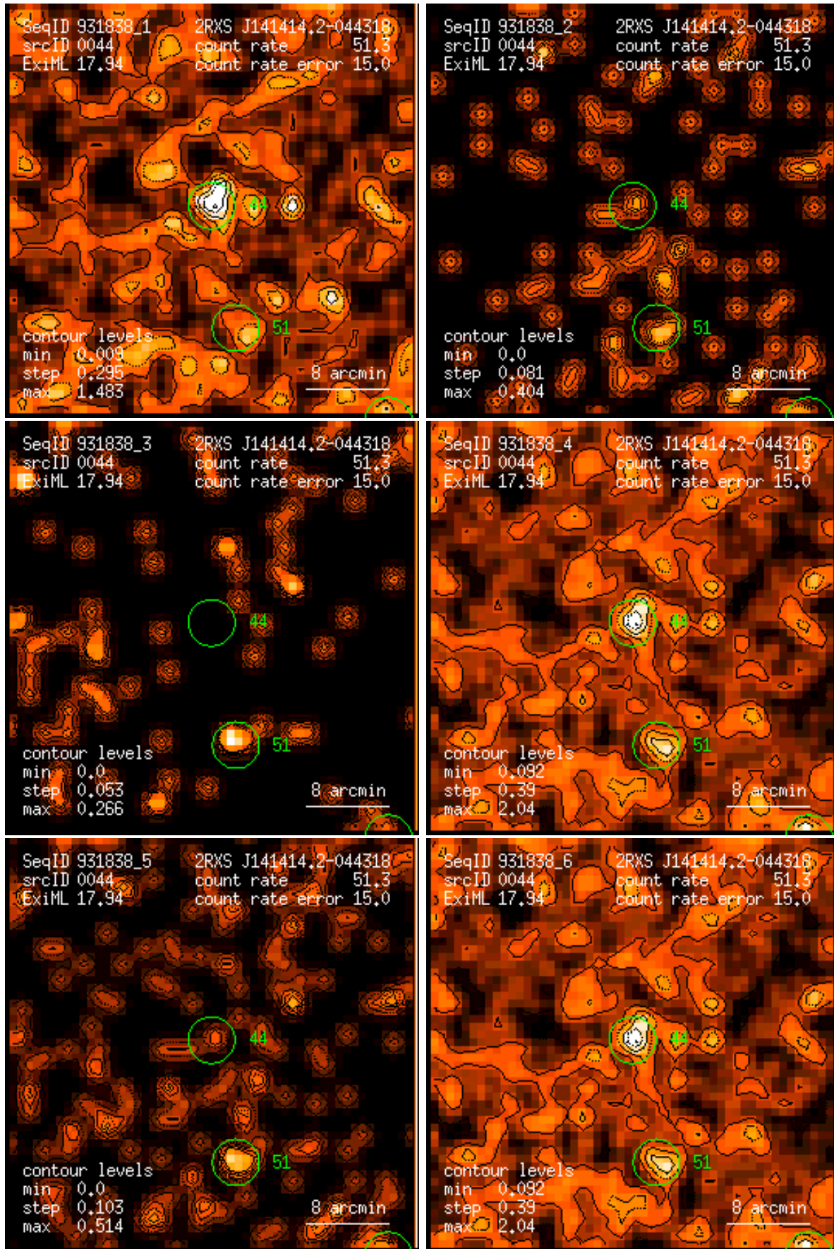
Figure 44: RASS 931838: detection 0044: band rate images, Gaussian filter: (1) PSPC channels 11 – 41, (2) 52 – 90, (3) 91 – 201, (4) 11 – 235, (5) 52 – 201, (6) 11 – 201. Broad band rates in counts/ks. Band rate contour levels in counts/ks/arcmin 2 .
