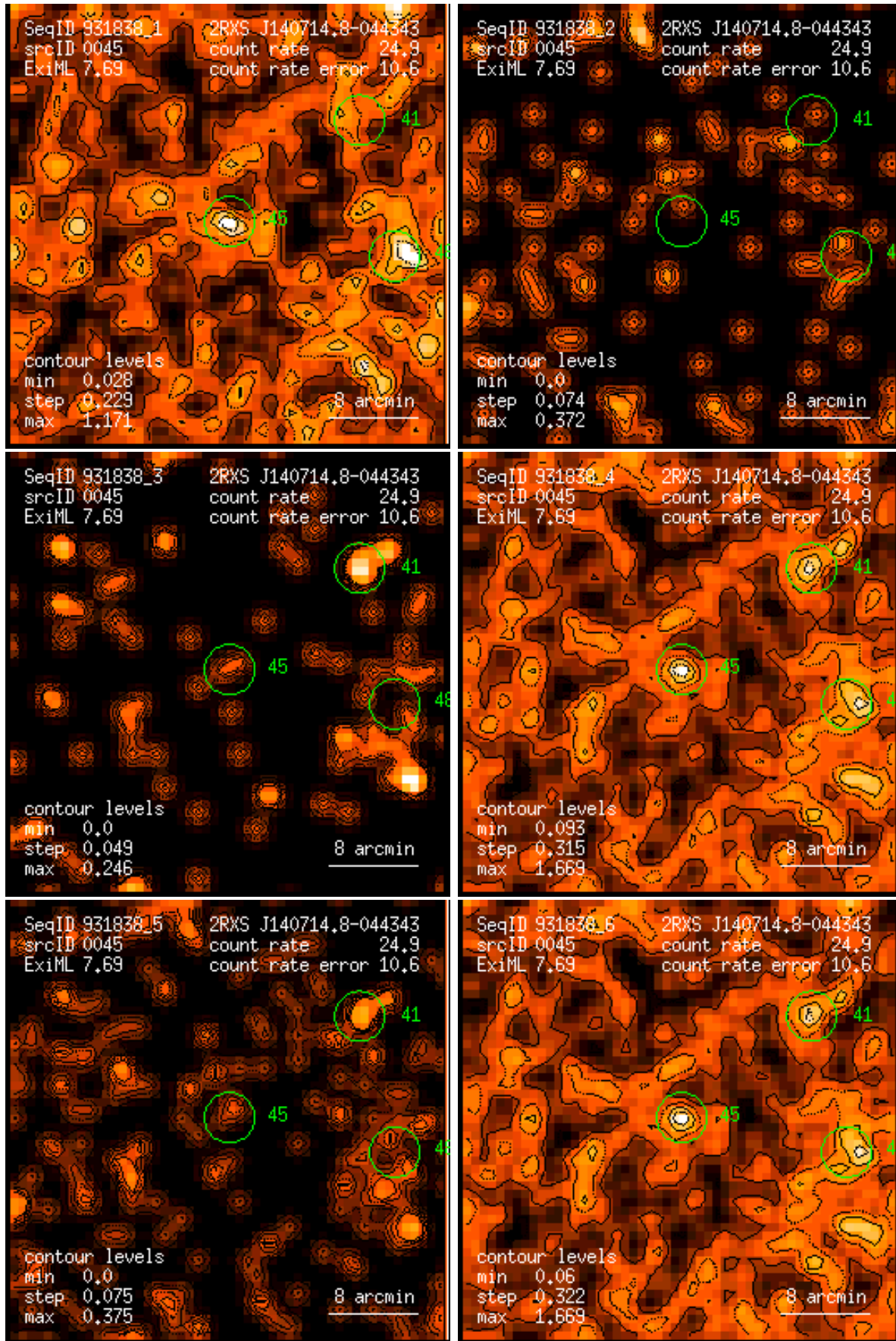
Figure 45: RASS 931838: detection 0045: band rate images, Gaussian filter: (1) PSPC channels 11 – 41, (2) 52 – 90, (3) 91 – 201, (4) 11 – 235, (5) 52 – 201, (6) 11 – 201. Broad band rates in counts/ks. Band rate contour levels in counts/ks/arcmin 2 .
