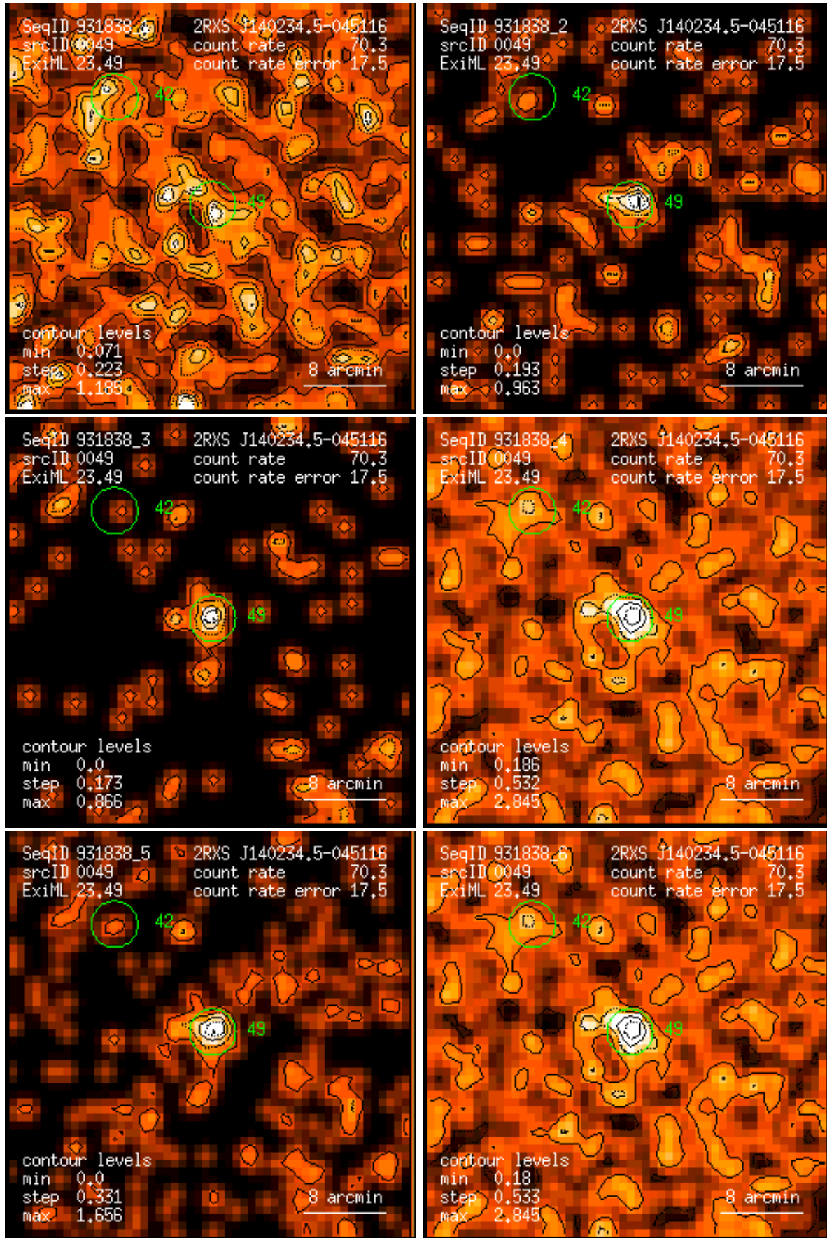
Figure 49: RASS 931838: detection 0049: band rate images, Gaussian filter: (1) PSPC channels 11 – 41, (2) 52 – 90, (3) 91 – 201, (4) 11 – 235, (5) 52 – 201, (6) 11 – 201. Broad band rates in counts/ks. Band rate contour levels in counts/ks/arcmin 2 .
