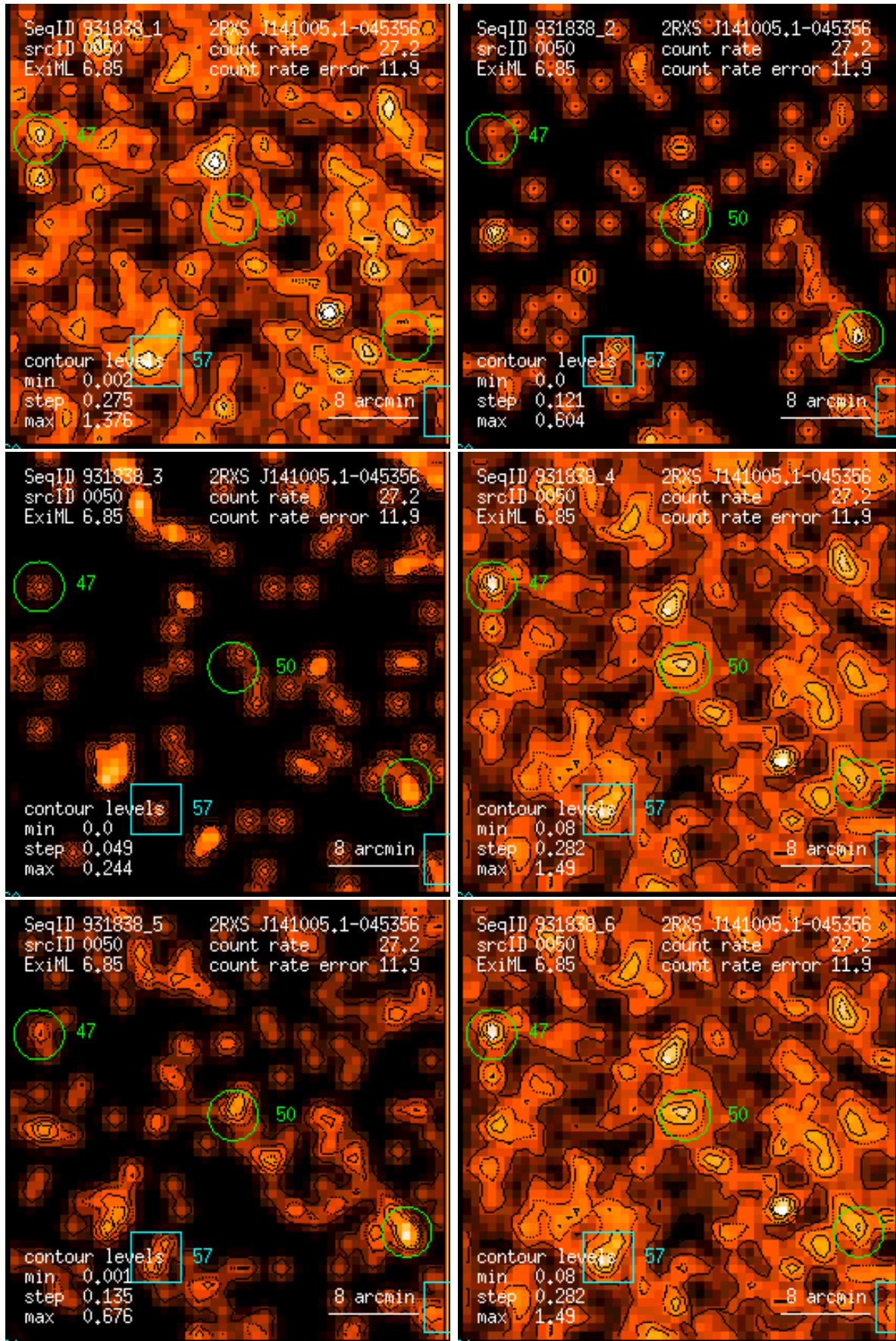
Figure 50: RASS 931838: detection 0050: band rate images, Gaussian filter: (1) PSPC channels 11 – 41, (2) 52 – 90, (3) 91 – 201, (4) 11 – 235, (5) 52 – 201, (6) 11 – 201. Broad band rates in counts/ks. Band rate contour levels in counts/ks/arcmin 2 .
