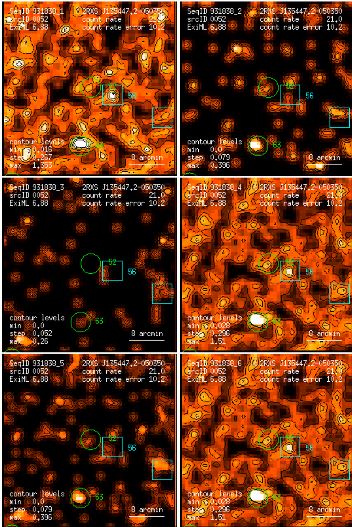
Figure 52: RASS 931838: detection 0052: band rate images, Gaussian filter: (1) PSPC channels 11 – 41, (2) 52 – 90, (3) 91 – 201, (4) 11 – 235, (5) 52 – 201, (6) 11 – 201. Broad band rates in counts/ks. Band rate contour levels in counts/ks/arcmin 2 .
