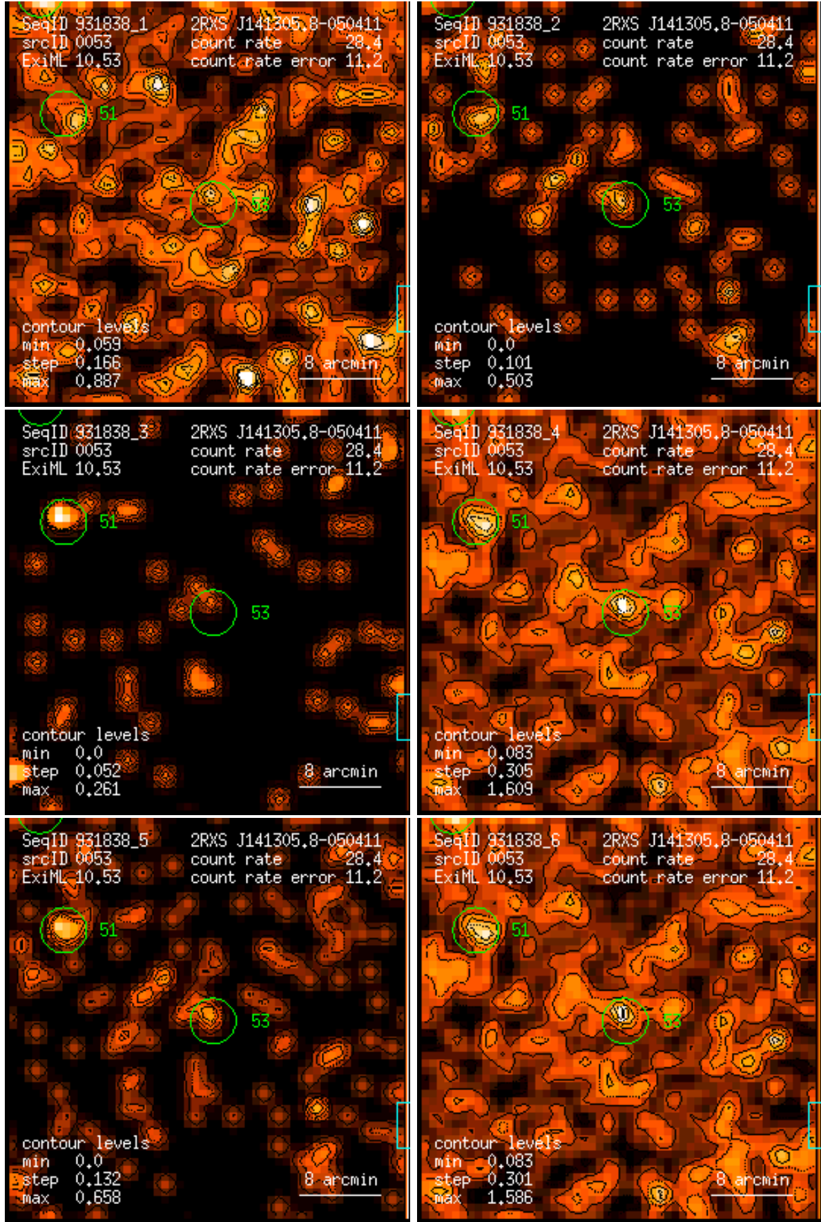
Figure 53: RASS 931838: detection 0053: band rate images, Gaussian filter: (1) PSPC channels 11 – 41, (2) 52 – 90, (3) 91 – 201, (4) 11 – 235, (5) 52 – 201, (6) 11 – 201. Broad band rates in counts/ks. Band rate contour levels in counts/ks/arcmin 2 .
