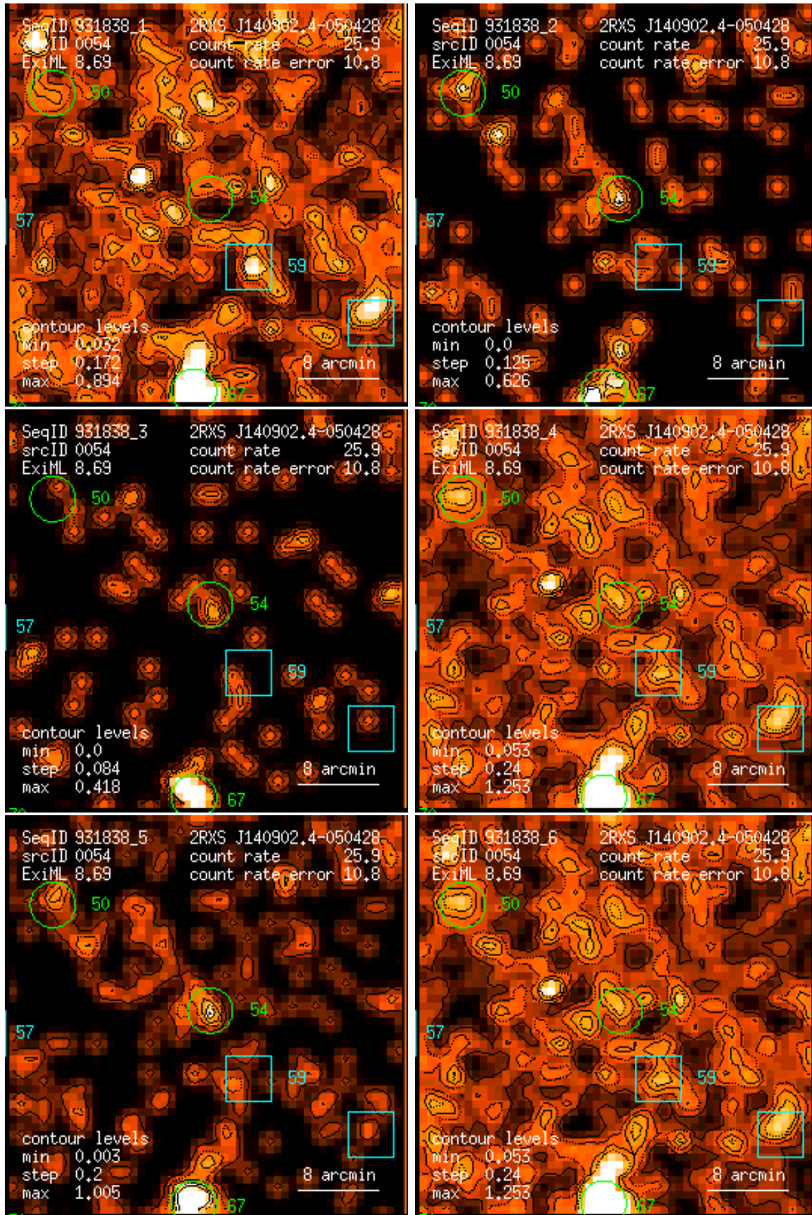
Figure 54: RASS 931838: detection 0054: band rate images, Gaussian filter: (1) PSPC channels 11 – 41, (2) 52 – 90, (3) 91 – 201, (4) 11 – 235, (5) 52 – 201, (6) 11 – 201. Broad band rates in counts/ks. Band rate contour levels in counts/ks/arcmin 2 .
