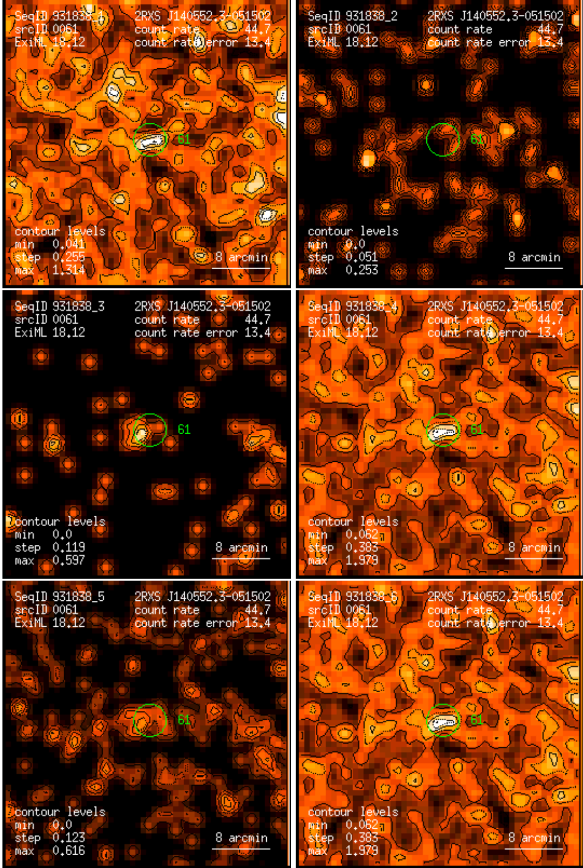
Figure 61: RASS 931838: detection 0061: band rate images, Gaussian filter: (1) PSPC channels 11 – 41, (2) 52 – 90, (3) 91 – 201, (4) 11 – 235, (5) 52 – 201, (6) 11 – 201. Broad band rates in counts/ks. Band rate contour levels in counts/ks/arcmin 2 .
