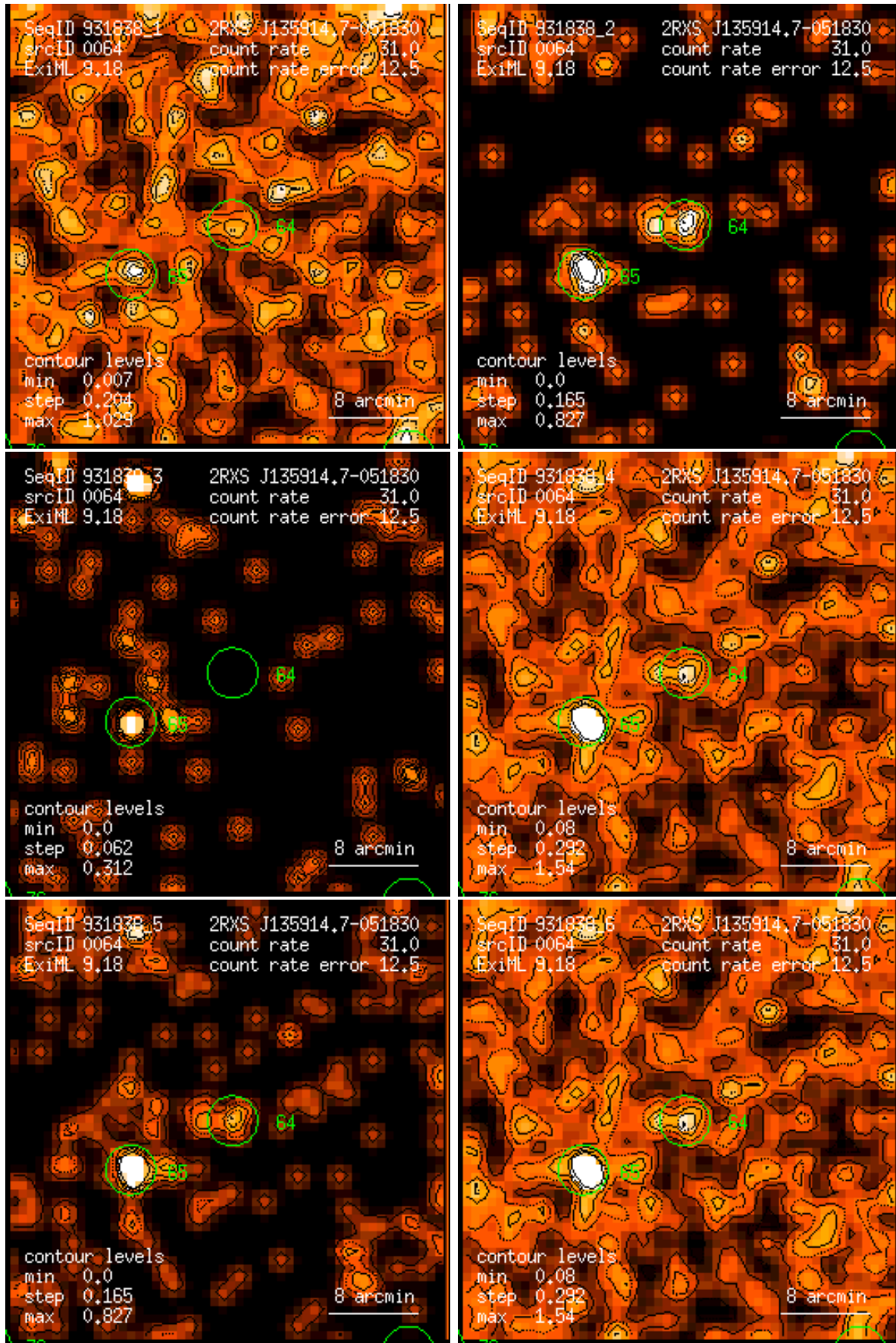
Figure 64: RASS 931838: detection 0064: band rate images, Gaussian filter: (1) PSPC channels 11 – 41, (2) 52 – 90, (3) 91 – 201, (4) 11 – 235, (5) 52 – 201, (6) 11 – 201. Broad band rates in counts/ks. Band rate contour levels in counts/ks/arcmin 2 .
