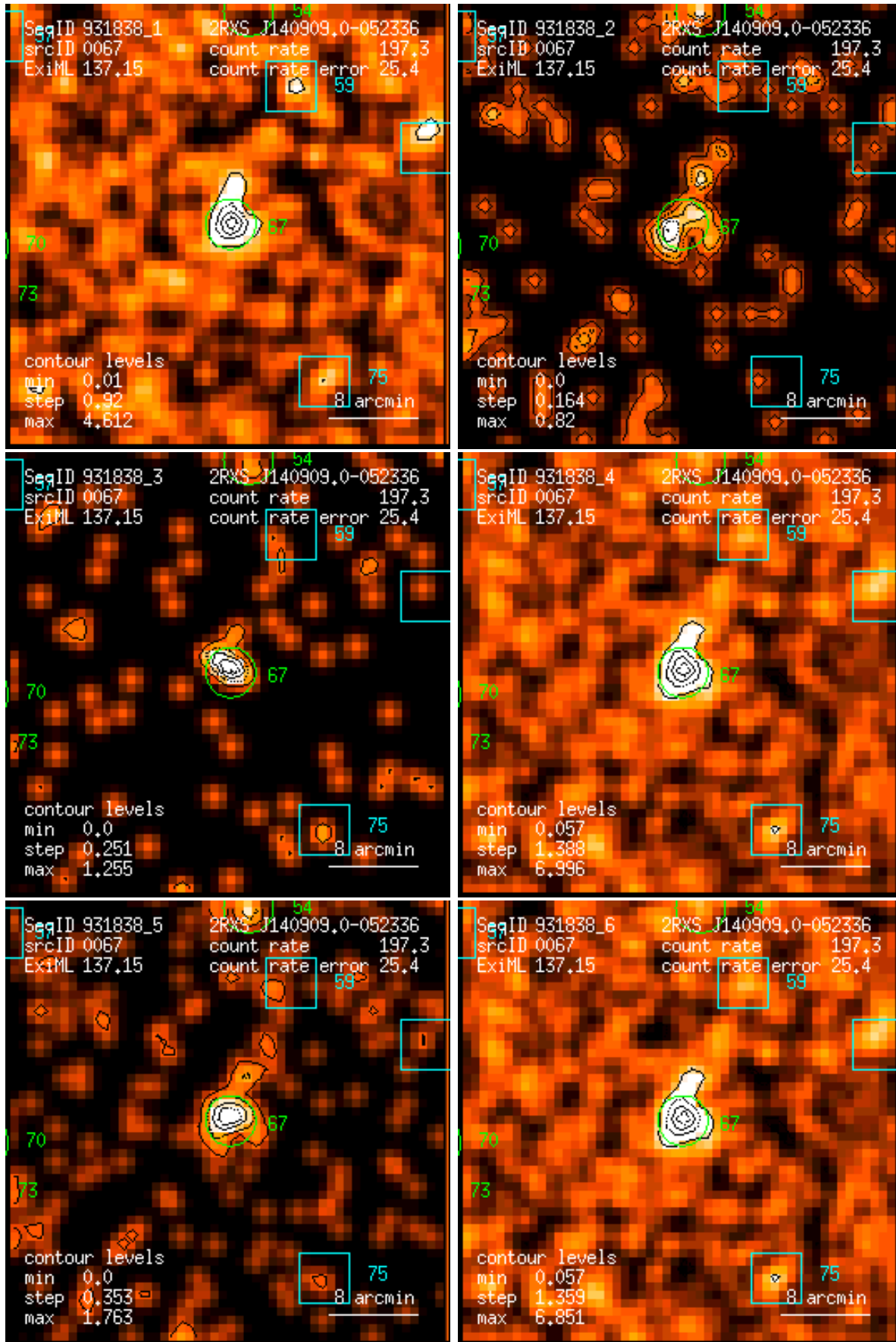
Figure 67: RASS 931838: detection 0067: band rate images, Gaussian filter: (1) PSPC channels 11 – 41, (2) 52 – 90, (3) 91 – 201, (4) 11 – 235, (5) 52 – 201, (6) 11 – 201. Broad band rates in counts/ks. Band rate contour levels in counts/ks/arcmin 2 .
