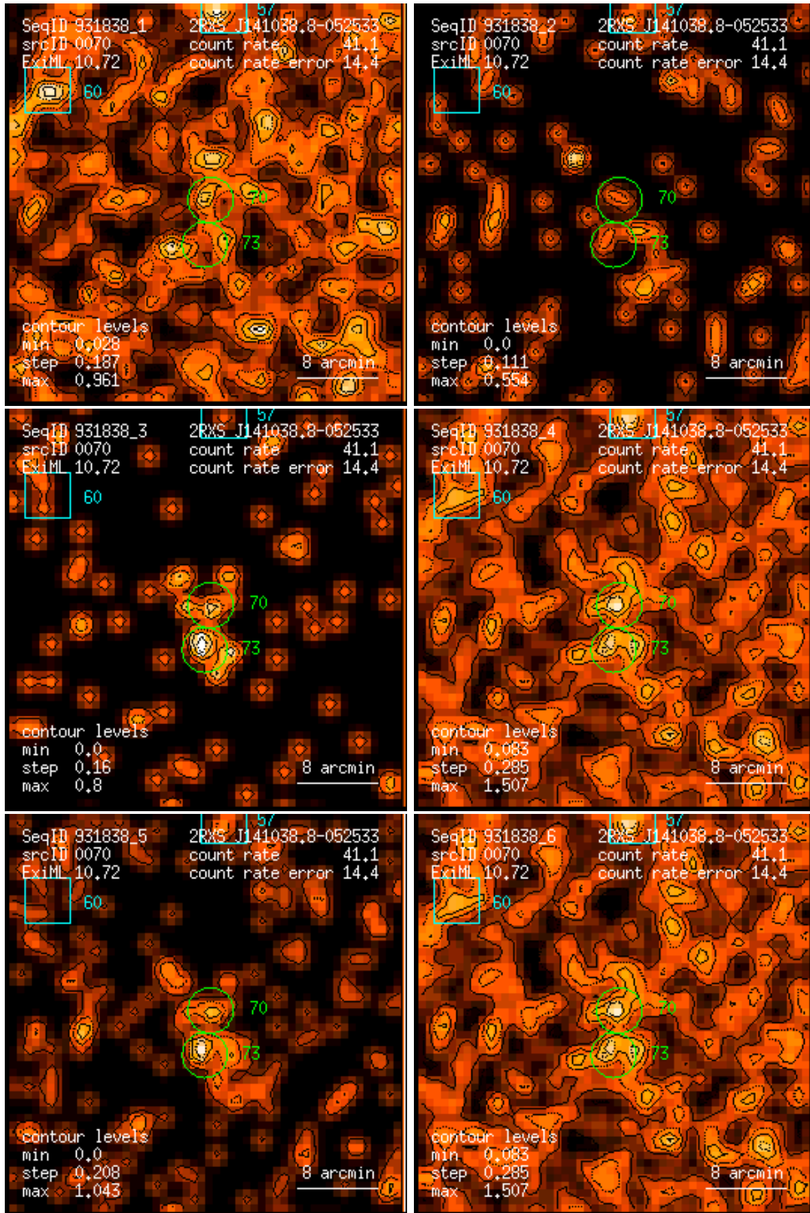
Figure 70: RASS 931838: detection 0070: band rate images, Gaussian filter: (1) PSPC channels 11 – 41, (2) 52 – 90, (3) 91 – 201, (4) 11 – 235, (5) 52 – 201, (6) 11 – 201. Broad band rates in counts/ks. Band rate contour levels in counts/ks/arcmin 2 .
