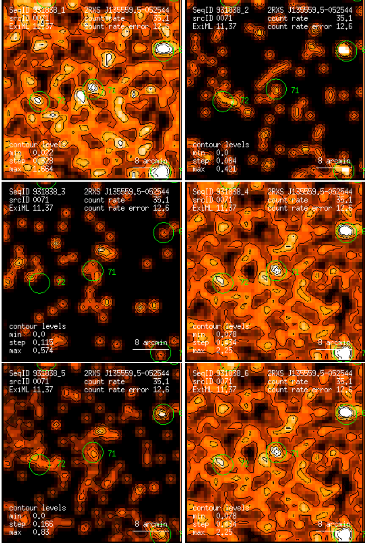
Figure 71: RASS 931838: detection 0071: band rate images, Gaussian filter: (1) PSPC channels 11 – 41, (2) 52 – 90, (3) 91 – 201, (4) 11 – 235, (5) 52 – 201, (6) 11 – 201. Broad band rates in counts/ks. Band rate contour levels in counts/ks/arcmin 2 .
