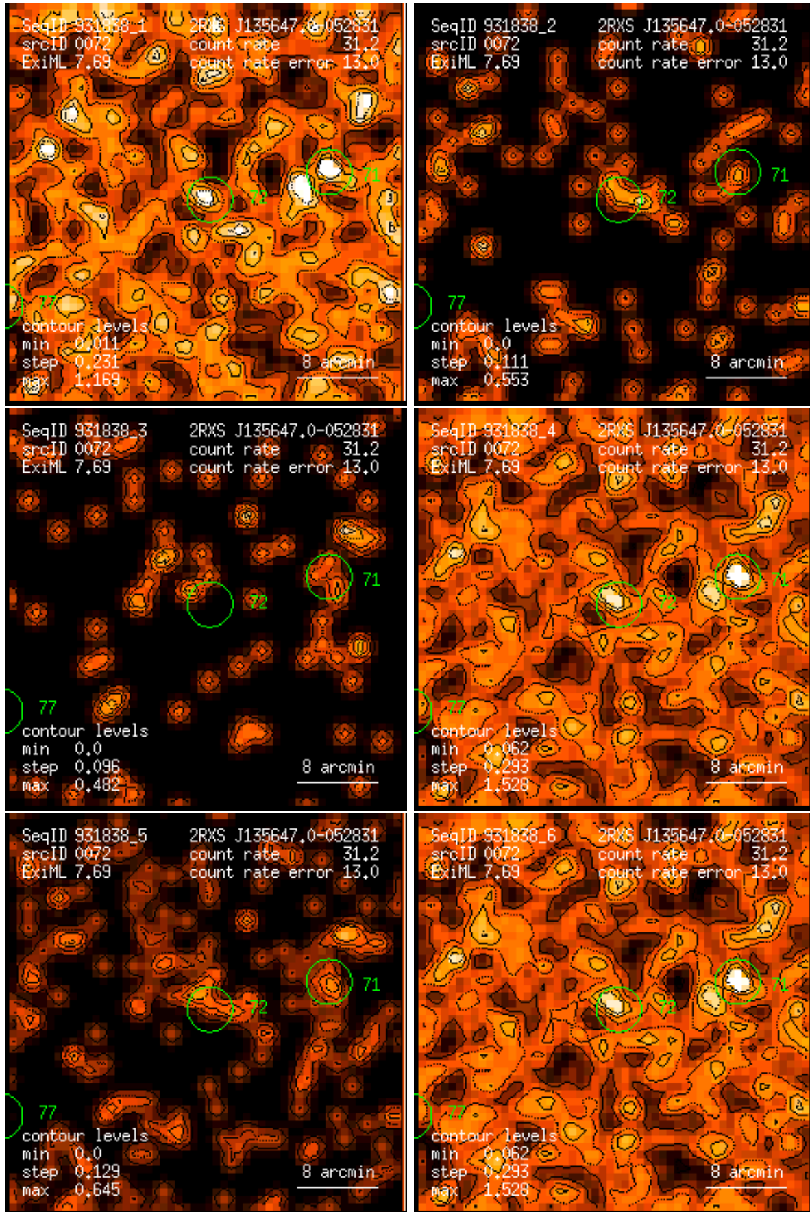
Figure 72: RASS 931838: detection 0072: band rate images, Gaussian filter: (1) PSPC channels 11 – 41, (2) 52 – 90, (3) 91 – 201, (4) 11 – 235, (5) 52 – 201, (6) 11 – 201. Broad band rates in counts/ks. Band rate contour levels in counts/ks/arcmin 2 .
