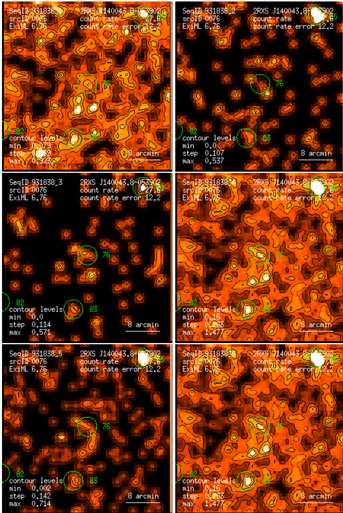
Figure 76: RASS 931838: detection 0076: band rate images, Gaussian filter: (1) PSPC channels 11 – 41, (2) 52 – 90, (3) 91 – 201, (4) 11 – 235, (5) 52 – 201, (6) 11 – 201. Broad band rates in counts/ks. Band rate contour levels in counts/ks/arcmin 2 .
