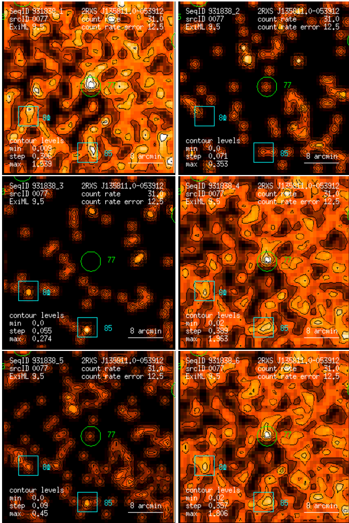
Figure 77: RASS 931838: detection 0077: band rate images, Gaussian filter: (1) PSPC channels 11 – 41, (2) 52 – 90, (3) 91 – 201, (4) 11 – 235, (5) 52 – 201, (6) 11 – 201. Broad band rates in counts/ks. Band rate contour levels in counts/ks/arcmin 2 .
