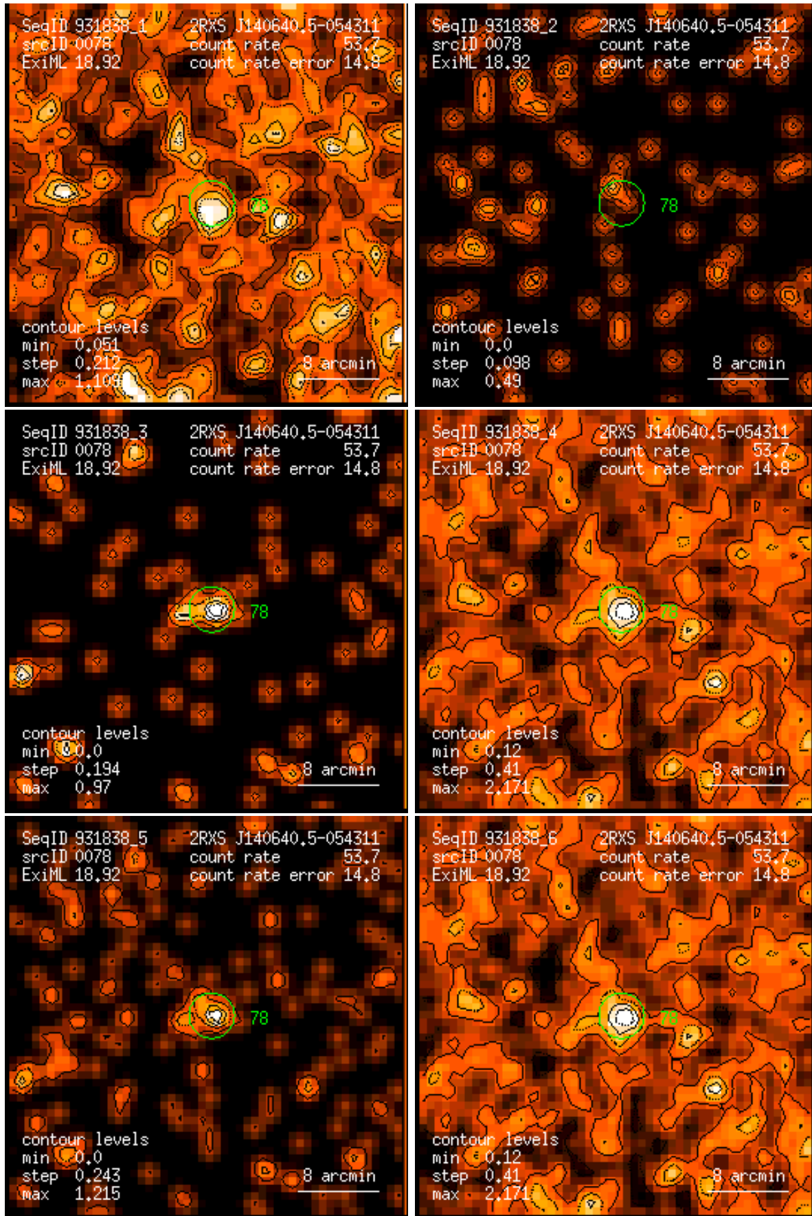
Figure 78: RASS 931838: detection 0078: band rate images, Gaussian filter: (1) PSPC channels 11 – 41, (2) 52 – 90, (3) 91 – 201, (4) 11 – 235, (5) 52 – 201, (6) 11 – 201. Broad band rates in counts/ks. Band rate contour levels in counts/ks/arcmin 2 .
