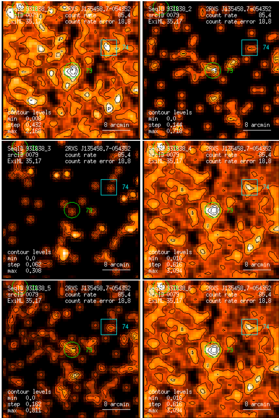
Figure 79: RASS 931838: detection 0079: band rate images, Gaussian filter: (1) PSPC channels 11 – 41, (2) 52 – 90, (3) 91 – 201, (4) 11 – 235, (5) 52 – 201, (6) 11 – 201. Broad band rates in counts/ks. Band rate contour levels in counts/ks/arcmin 2 .
