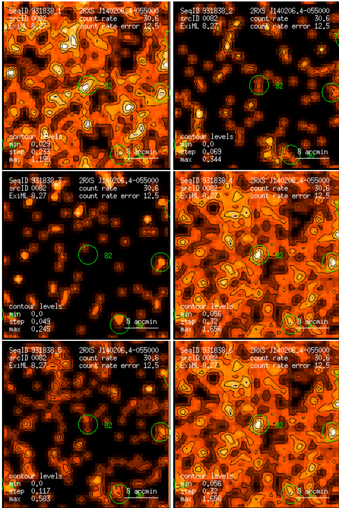
Figure 82: RASS 931838: detection 0082: band rate images, Gaussian filter: (1) PSPC channels 11 – 41, (2) 52 – 90, (3) 91 – 201, (4) 11 – 235, (5) 52 – 201, (6) 11 – 201. Broad band rates in counts/ks. Band rate contour levels in counts/ks/arcmin 2 .
