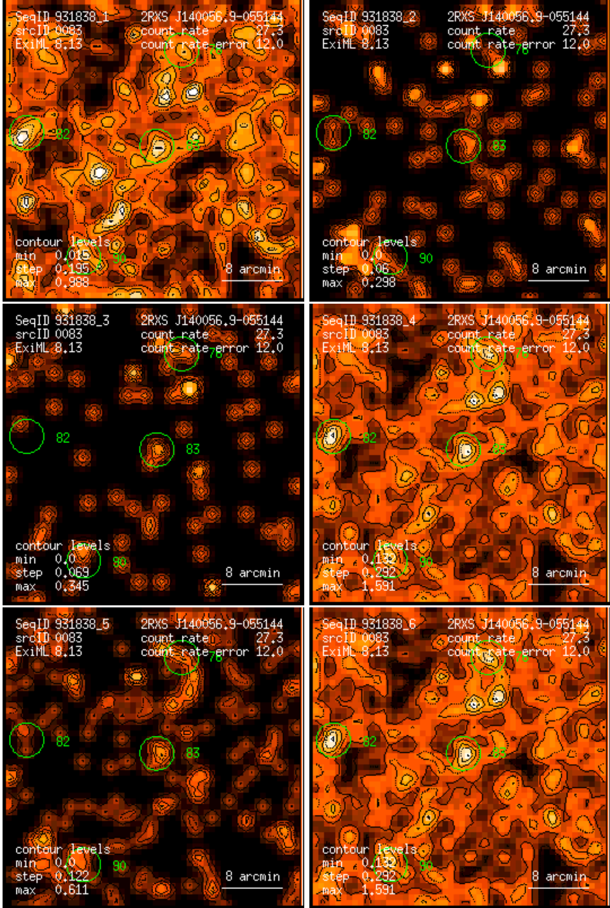
Figure 83: RASS 931838: detection 0083: band rate images, Gaussian filter: (1) PSPC channels 11 – 41, (2) 52 – 90, (3) 91 – 201, (4) 11 – 235, (5) 52 – 201, (6) 11 – 201. Broad band rates in counts/ks. Band rate contour levels in counts/ks/arcmin 2 .
