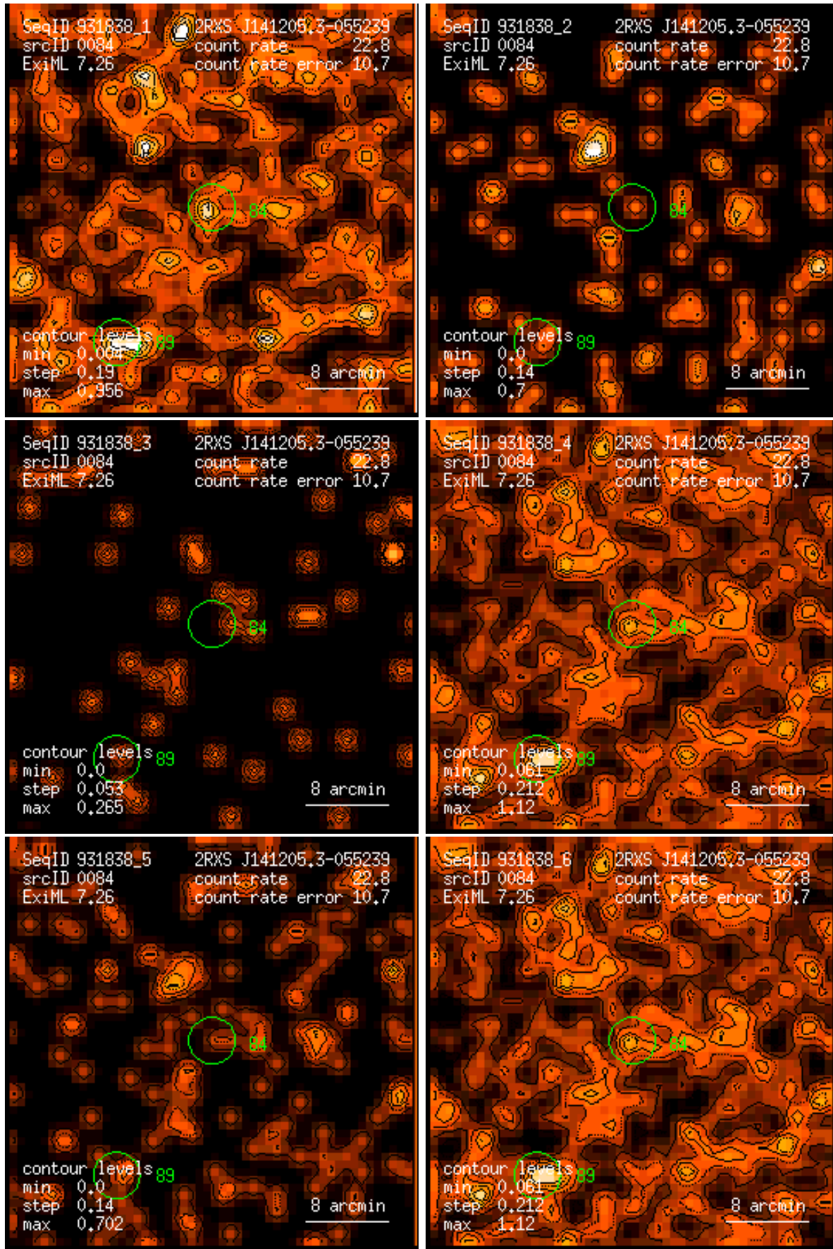
Figure 84: RASS 931838: detection 0084: band rate images, Gaussian filter: (1) PSPC channels 11 – 41, (2) 52 – 90, (3) 91 – 201, (4) 11 – 235, (5) 52 – 201, (6) 11 – 201. Broad band rates in counts/ks. Band rate contour levels in counts/ks/arcmin 2 .
