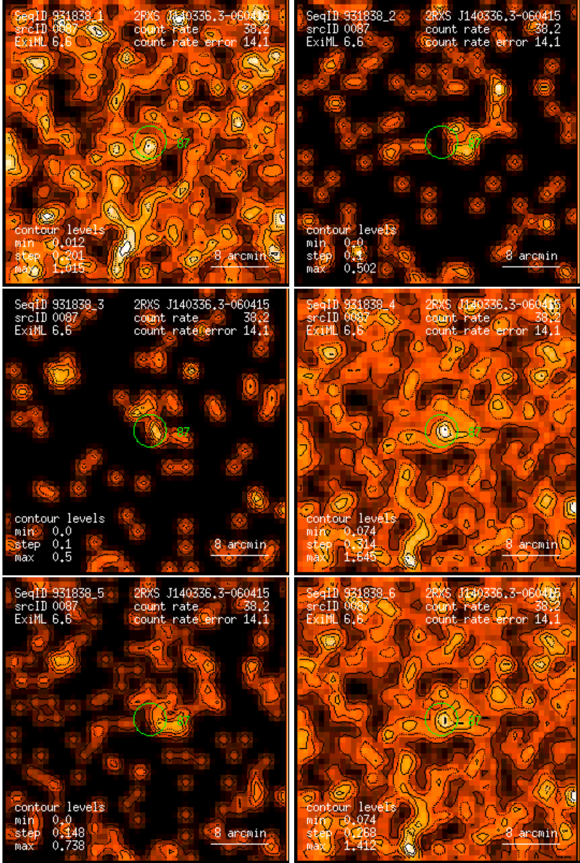
Figure 87: RASS 931838: detection 0087: band rate images, Gaussian filter: (1) PSPC channels 11 – 41, (2) 52 – 90, (3) 91 – 201, (4) 11 – 235, (5) 52 – 201, (6) 11 – 201. Broad band rates in counts/ks. Band rate contour levels in counts/ks/arcmin 2 .
