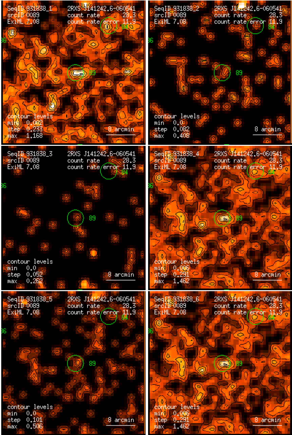
Figure 89: RASS 931838: detection 0089: band rate images, Gaussian filter: (1) PSPC channels 11 – 41, (2) 52 – 90, (3) 91 – 201, (4) 11 – 235, (5) 52 – 201, (6) 11 – 201. Broad band rates in counts/ks. Band rate contour levels in counts/ks/arcmin 2 .
