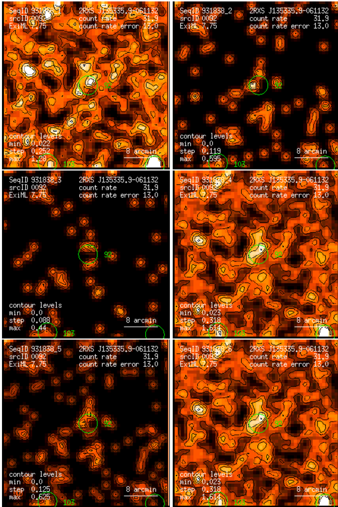
Figure 92: RASS 931838: detection 0092: band rate images, Gaussian filter: (1) PSPC channels 11 – 41, (2) 52 – 90, (3) 91 – 201, (4) 11 – 235, (5) 52 – 201, (6) 11 – 201. Broad band rates in counts/ks. Band rate contour levels in counts/ks/arcmin 2 .
