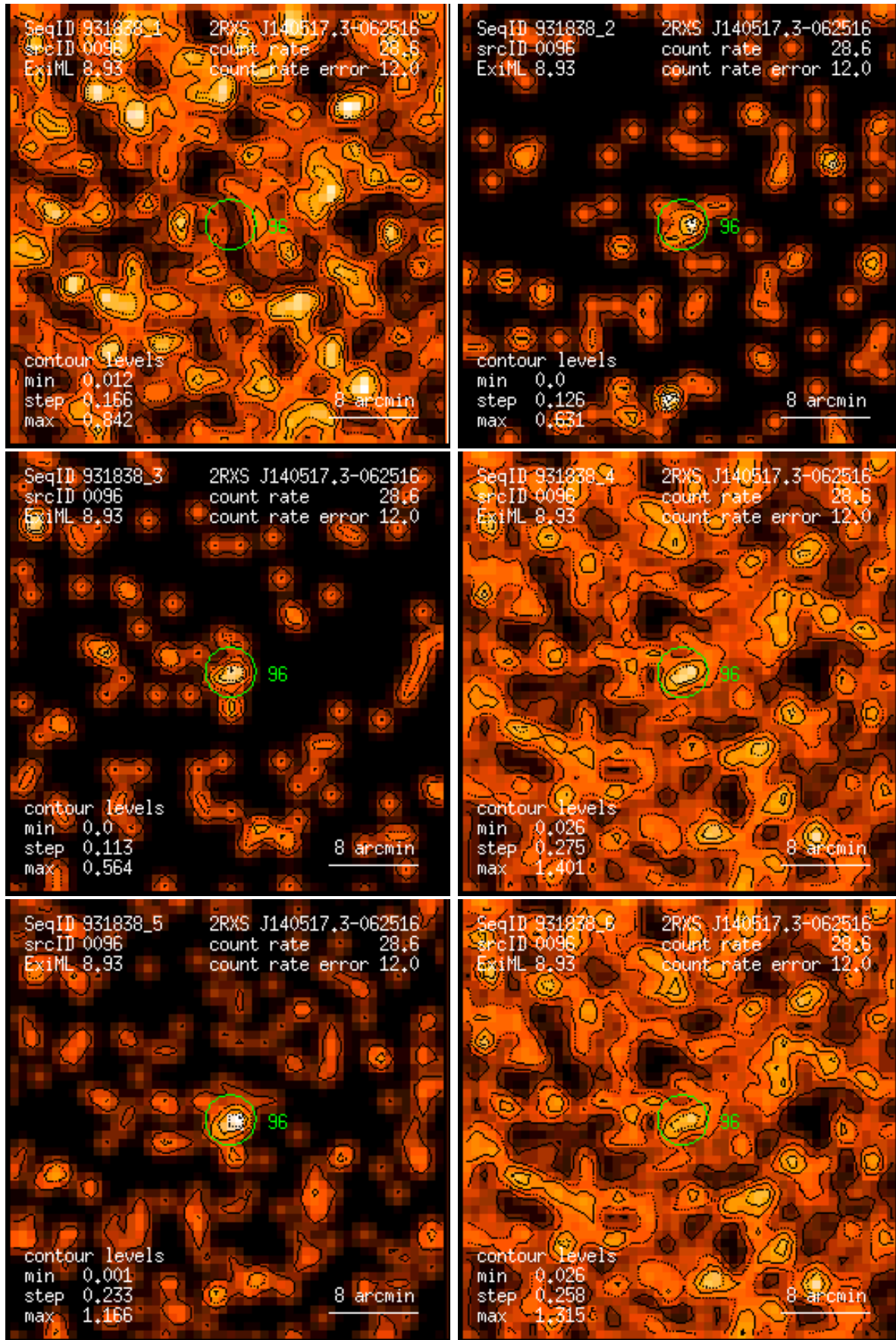
Figure 96: RASS 931838: detection 0096: band rate images, Gaussian filter: (1) PSPC channels 11 – 41, (2) 52 – 90, (3) 91 – 201, (4) 11 – 235, (5) 52 – 201, (6) 11 – 201. Broad band rates in counts/ks. Band rate contour levels in counts/ks/arcmin 2 .
