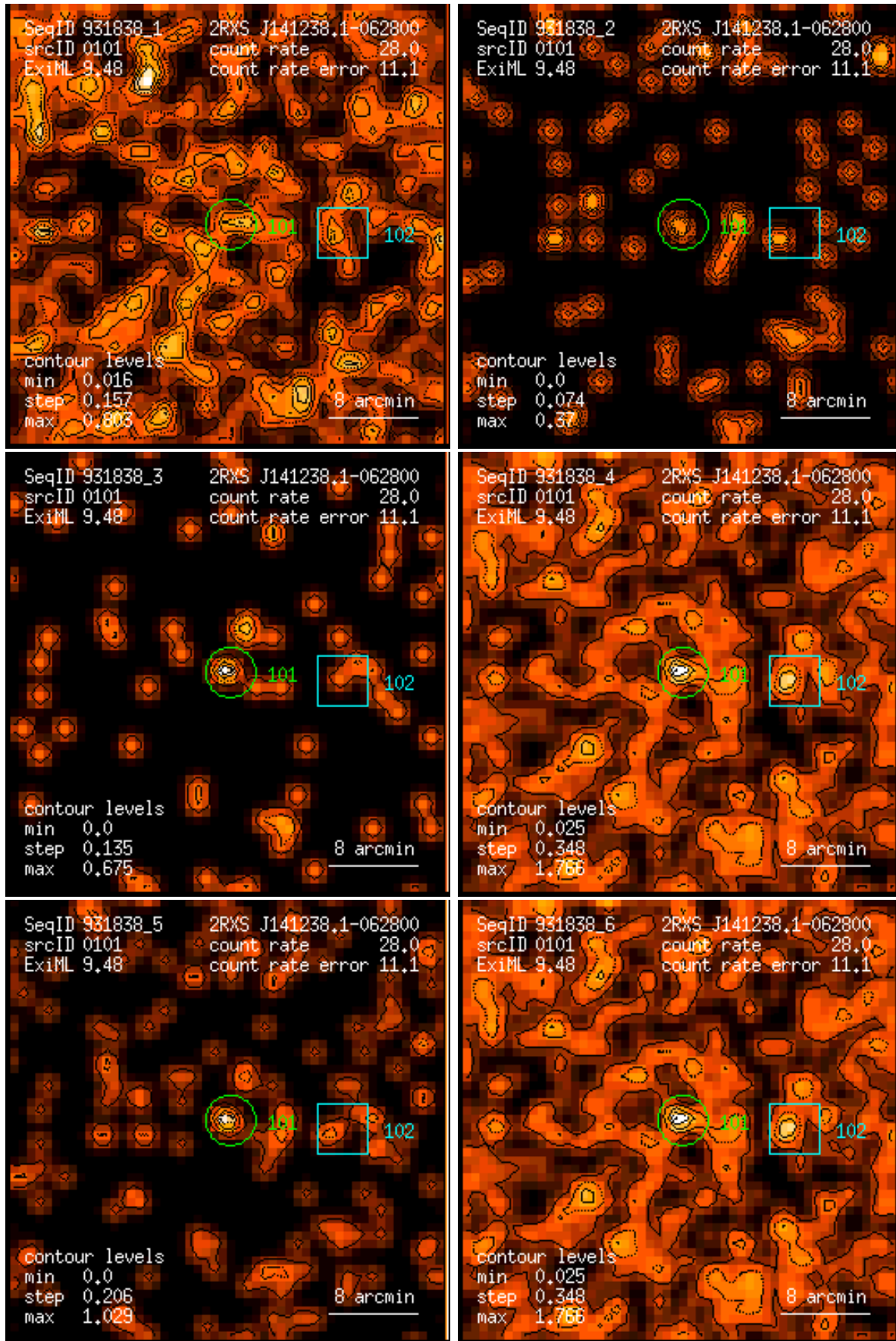
Figure 101: RASS 931838: detection 0101: band rate images, Gaussian filter: (1) PSPC channels 11 – 41, (2) 52 – 90, (3) 91 – 201, (4) 11 – 235, (5) 52 – 201, (6) 11 – 201. Broad band rates in counts/ks. Band rate contour levels in counts/ks/arcmin 2 .
